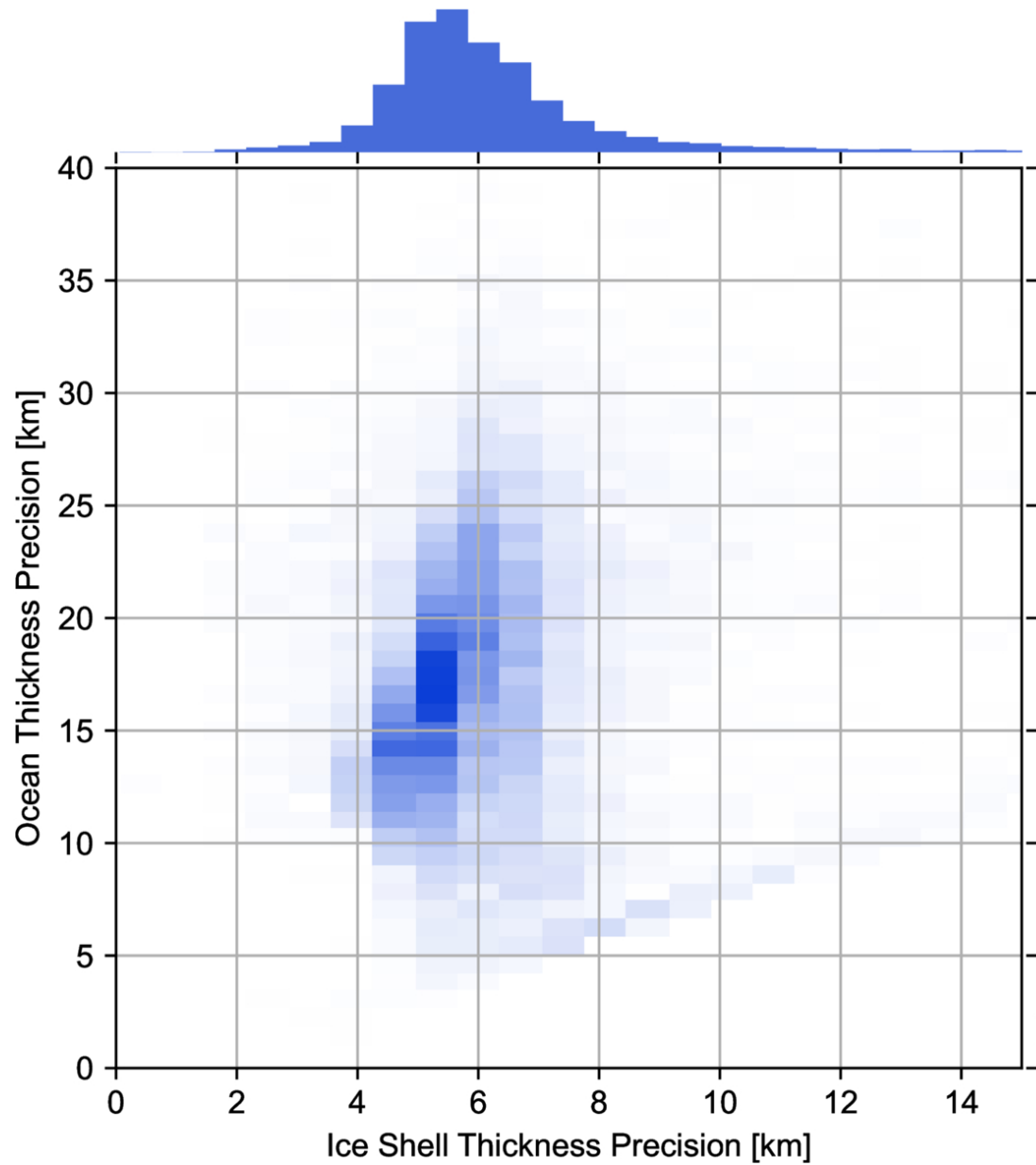
Figure 10. from Flavio Petricca et al 2026 Planet. Sci. J. 7 doi:10.3847/PSJ/ae5225 https://dx.doi.org/10.3847/PSJ/ae5225 © 2026. The Author(s). Published by the American Astronomical Society.
