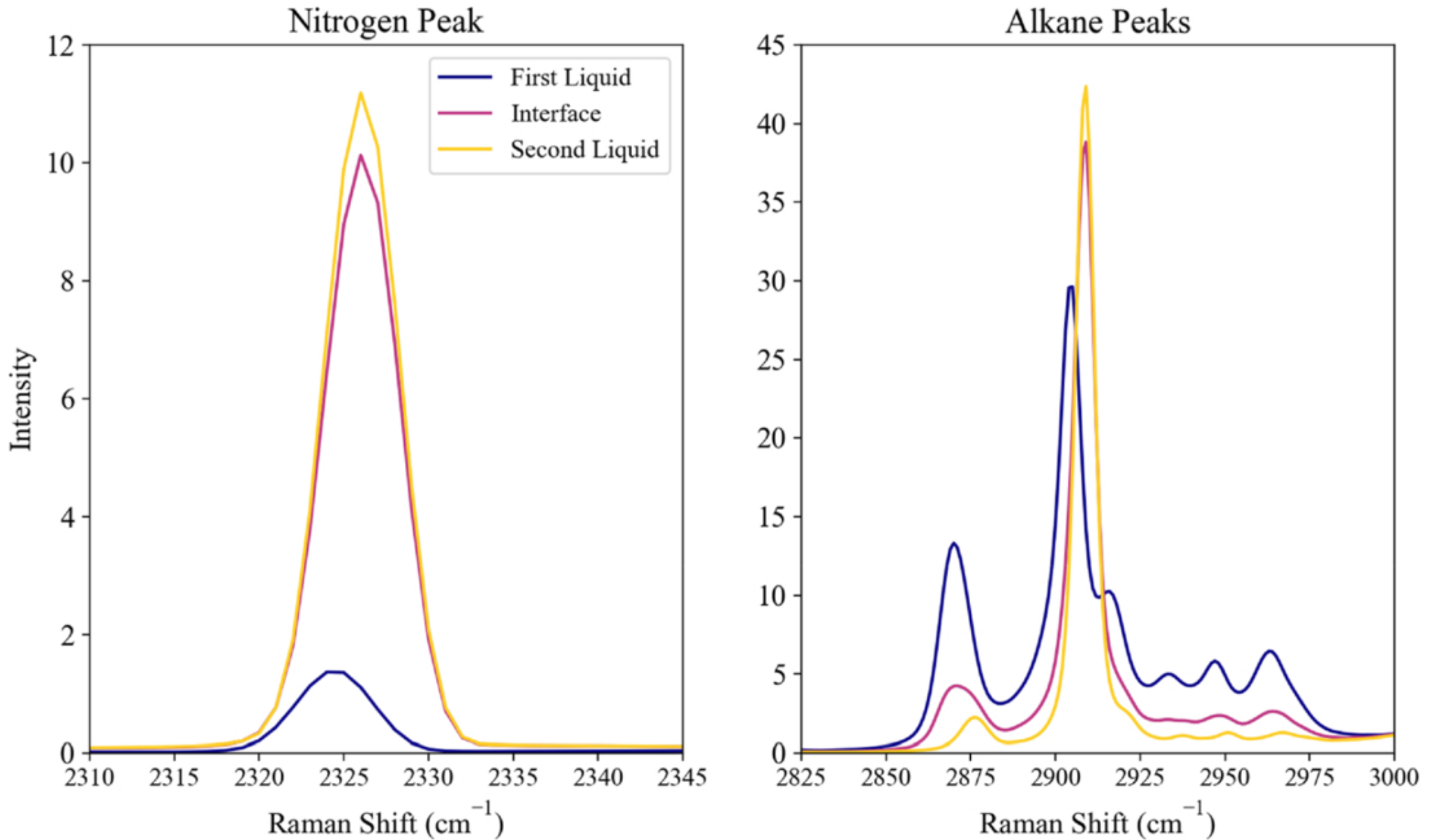
Figure 5. from Cecilia Thieberger et al 2026 Planet. Sci. J. 7 doi:10.3847/PSJ/ae4fb3 https://dx.doi.org/10.3847/PSJ/ae4fb3 © 2026. The Author(s). Published by the American Astronomical Society.
