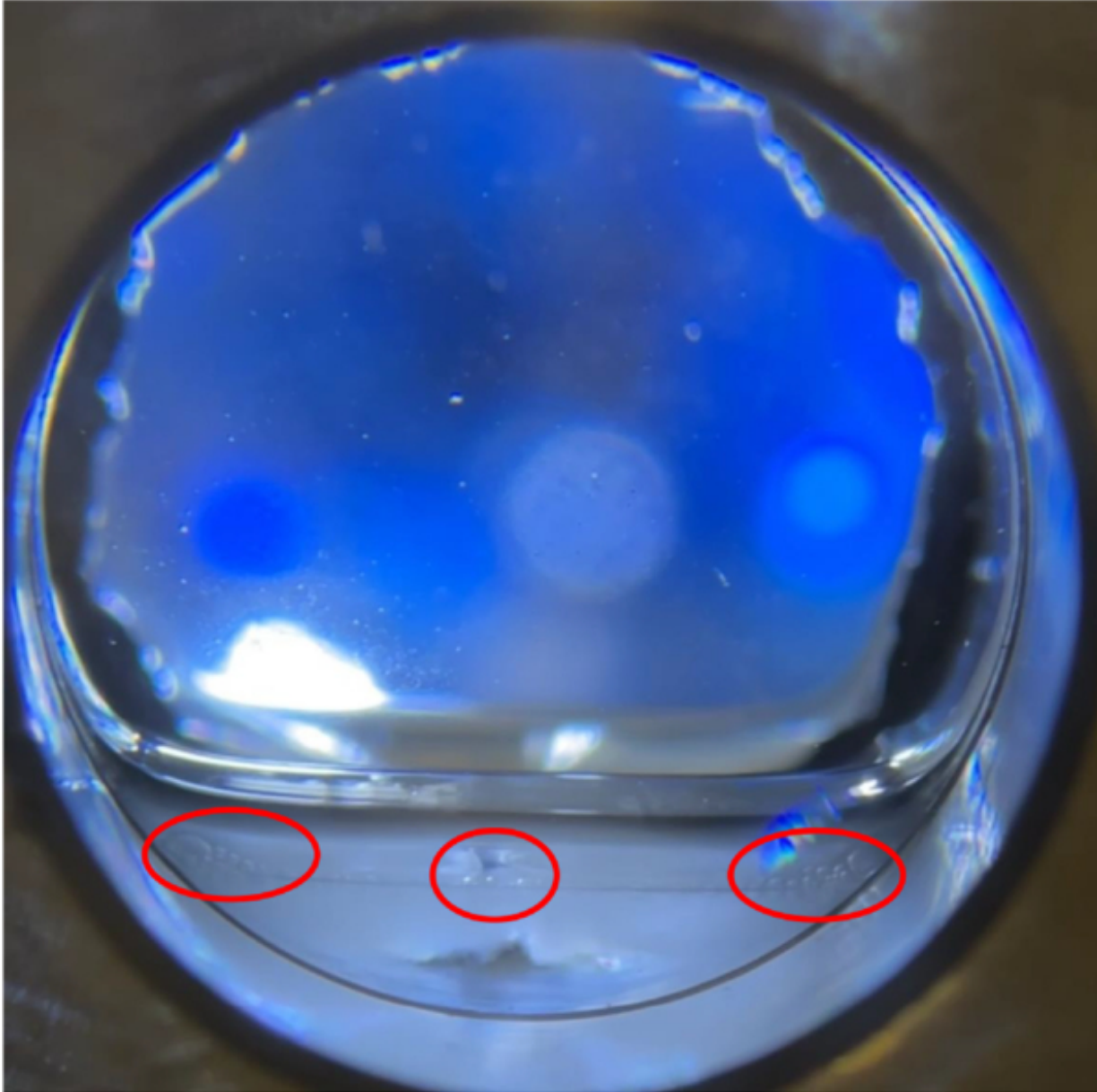
Figure 4. from Cecilia Thieberger et al 2026 Planet. Sci. J. 7 doi:10.3847/PSJ/ae4fb3 https://dx.doi.org/10.3847/PSJ/ae4fb3 © 2026. The Author(s). Published by the American Astronomical Society.
