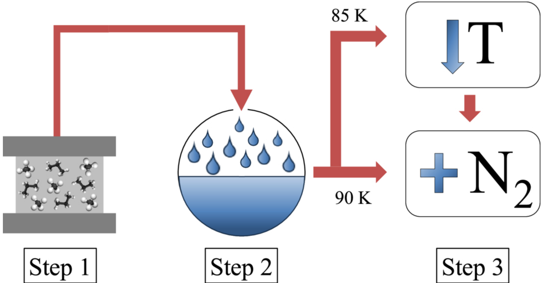
Figure 2. from Cecilia Thieberger et al 2026 Planet. Sci. J. 7 doi:10.3847/PSJ/ae4fb3 https://dx.doi.org/10.3847/PSJ/ae4fb3 © 2026. The Author(s). Published by the American Astronomical Society.
