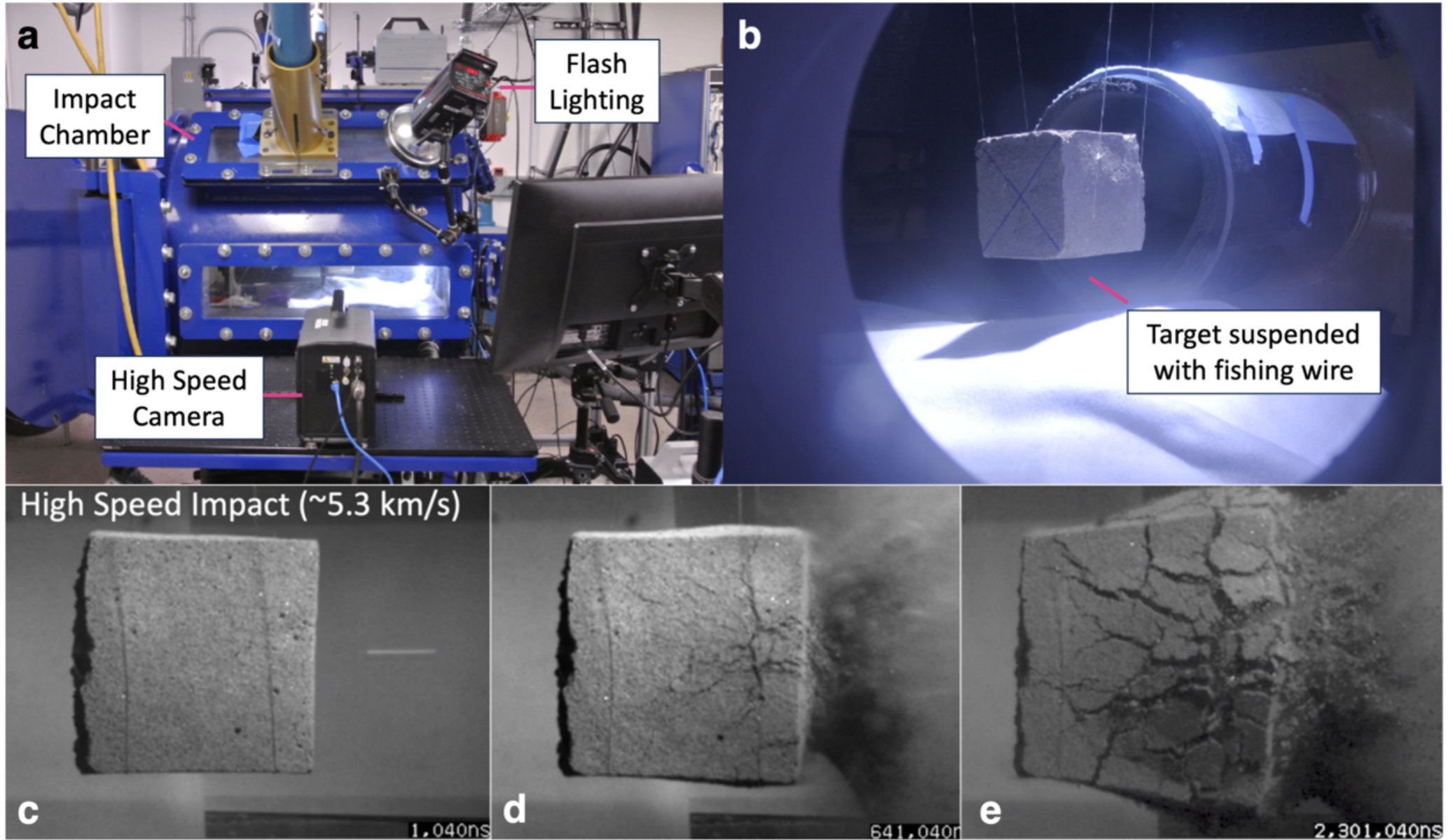
Figure 7. from R.-L. Ballouz et al 2026 Planet. Sci. J. 7 doi:10.3847/PSJ/ae4fad https://dx.doi.org/10.3847/PSJ/ae4fad © 2026. The Author(s). Published by the American Astronomical Society.
