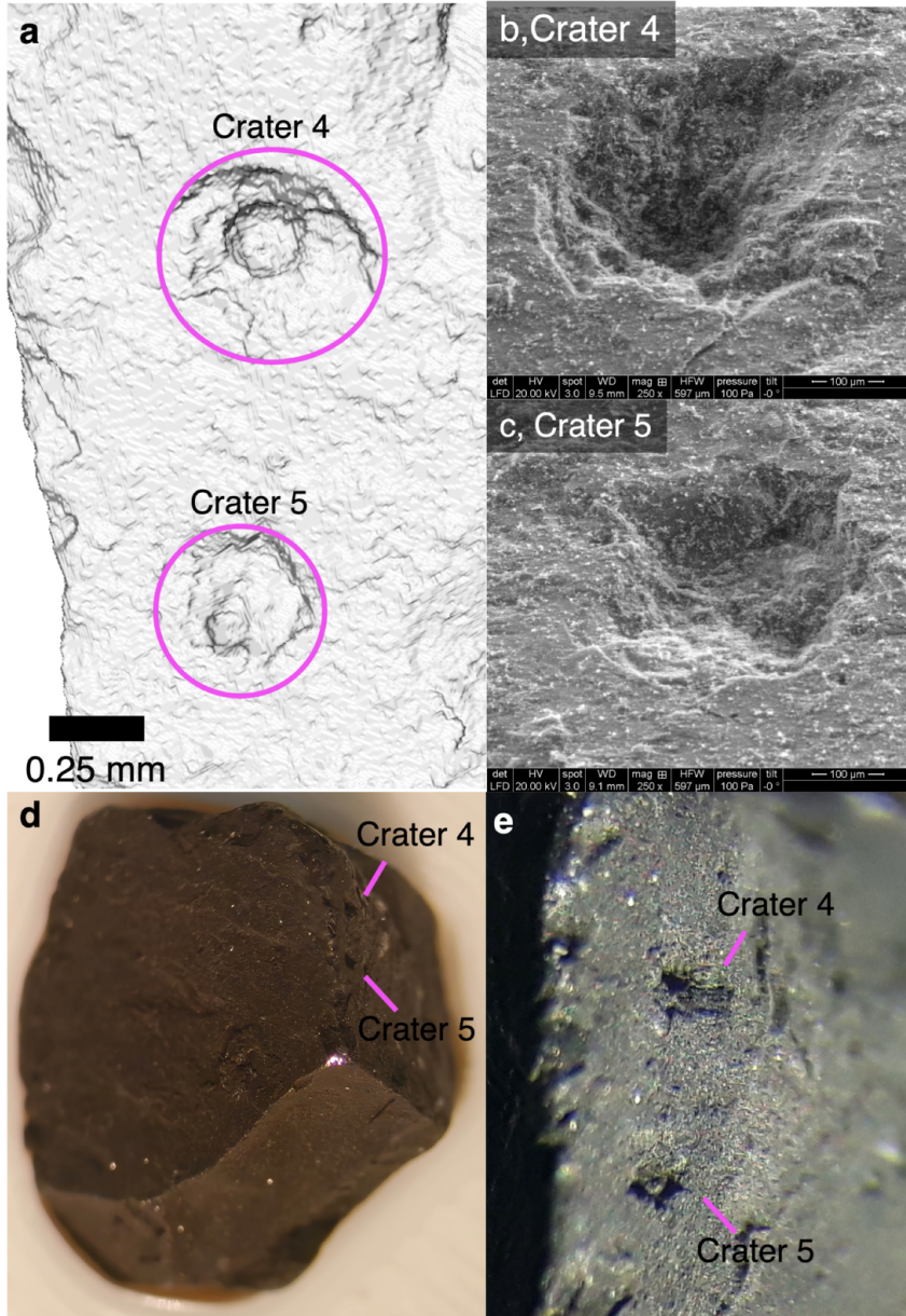
Figure 4. from R.-L. Ballouz et al 2026 Planet. Sci. J. 7 doi:10.3847/PSJ/ae4fad https://dx.doi.org/10.3847/PSJ/ae4fad © 2026. The Author(s). Published by the American Astronomical Society.
