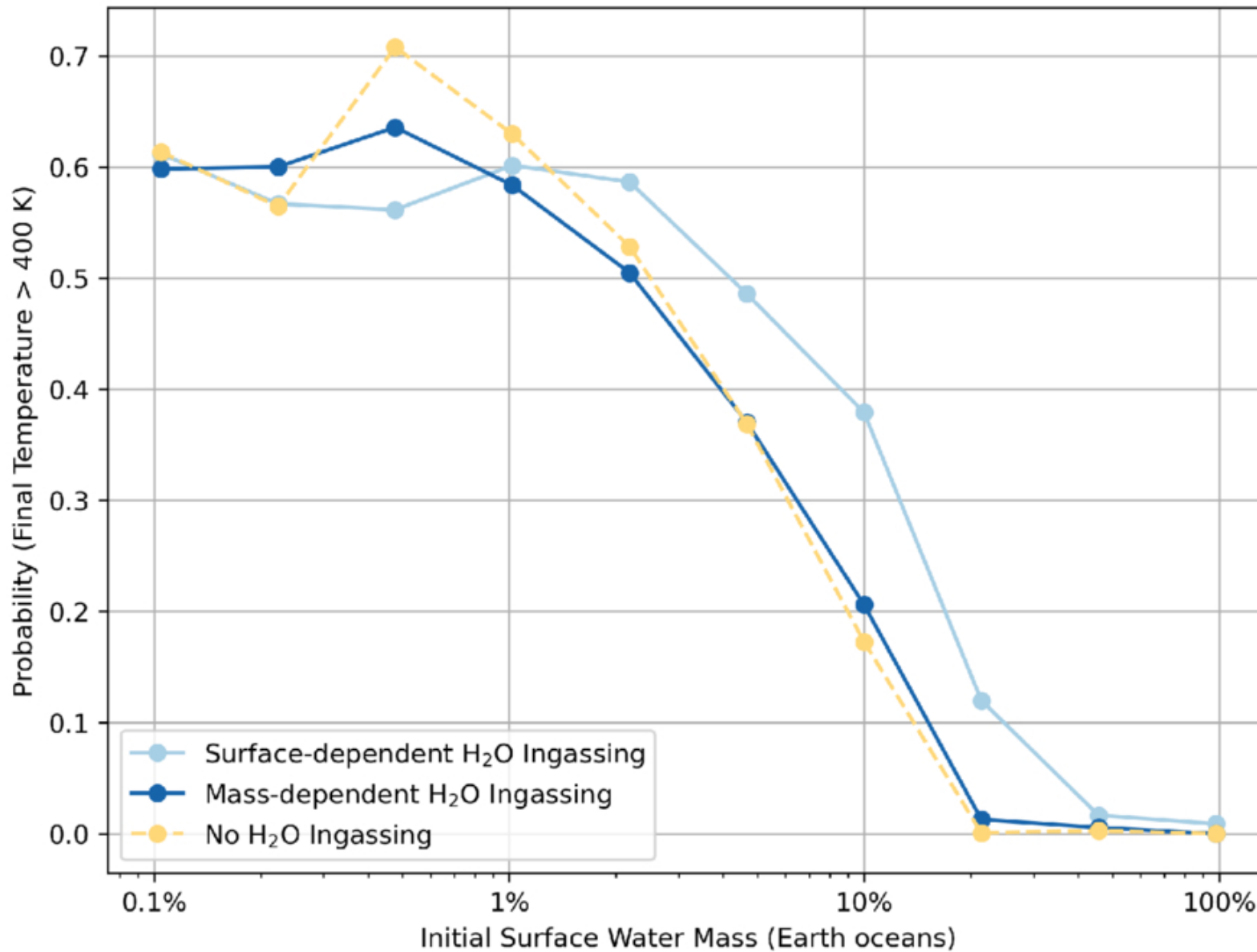
Figure 6. from Haskelle T. White-Gianella and Joshua Krissansen-Totton 2026 Planet. Sci. J. 7 doi:10.3847/PSJ/ae4faa https://dx.doi.org/10.3847/PSJ/ae4faa © 2026. The Author(s). Published by the American Astronomical Society.
