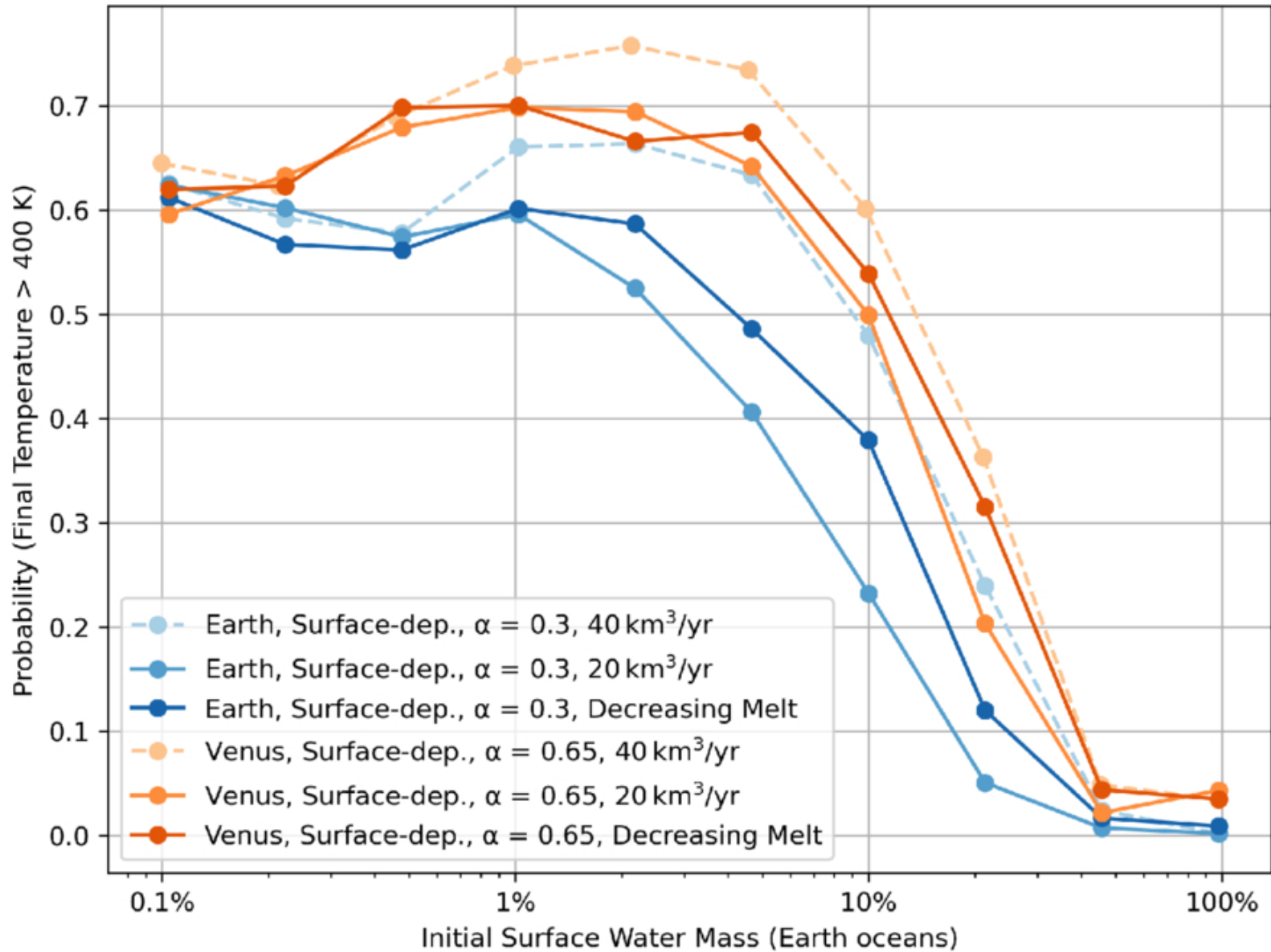
Figure A10. from Haskelle T. White-Gianella and Joshua Krissansen-Totton 2026 Planet. Sci. J. 7 doi:10.3847/PSJ/ae4faa https://dx.doi.org/10.3847/PSJ/ae4faa © 2026. The Author(s). Published by the American Astronomical Society.
