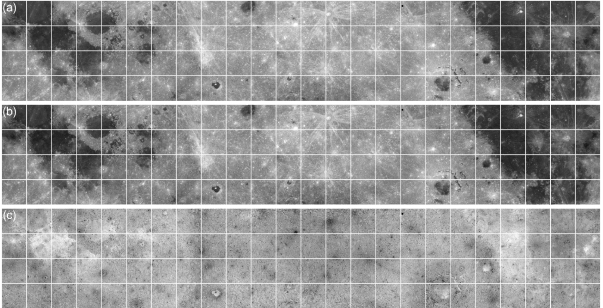
Figure 7. from Emerson Speyerer et al 2026 Planet. Sci. J. 7 doi:10.3847/PSJ/ae4a06 https://dx.doi.org/10.3847/PSJ/ae4a06 © 2026. The Author(s). Published by the American Astronomical Society.
