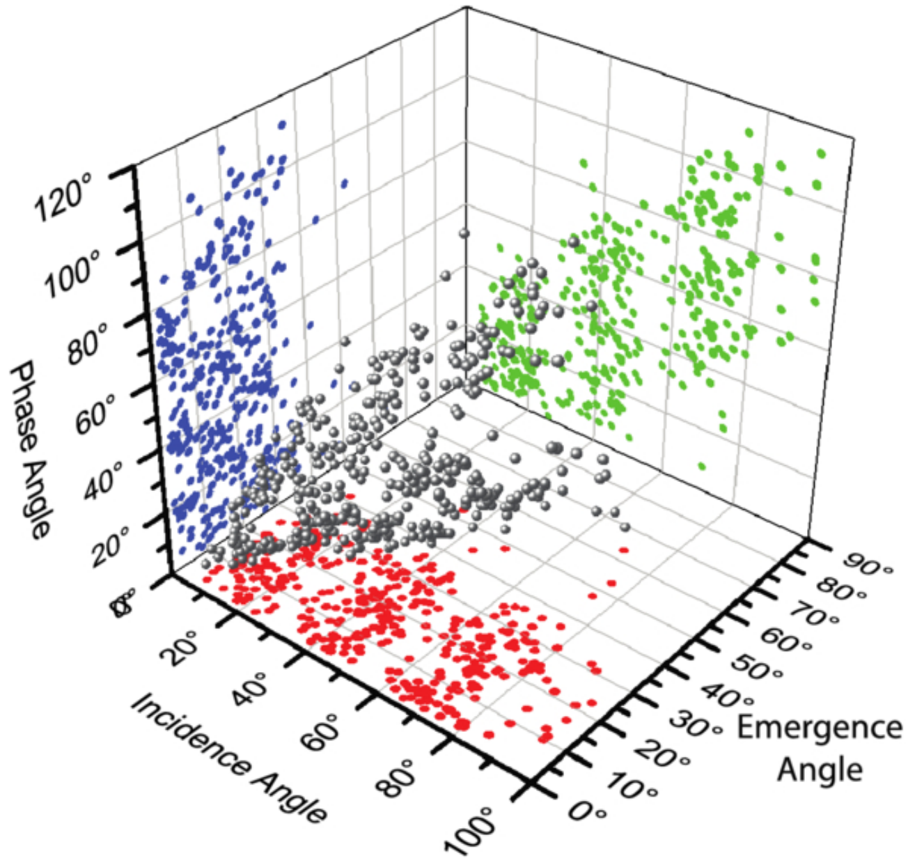
Figure 6. from Emerson Speyerer et al 2026 Planet. Sci. J. 7 doi:10.3847/PSJ/ae4a06 https://dx.doi.org/10.3847/PSJ/ae4a06 © 2026. The Author(s). Published by the American Astronomical Society.
