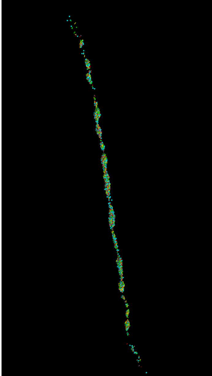
Figure 2. from Julian C. Marohnic et al 2026 Planet. Sci. J. 7 doi:10.3847/PSJ/ae4908 https://dx.doi.org/10.3847/PSJ/ae4908 © 2026. The Author(s). Published by the American Astronomical Society.
