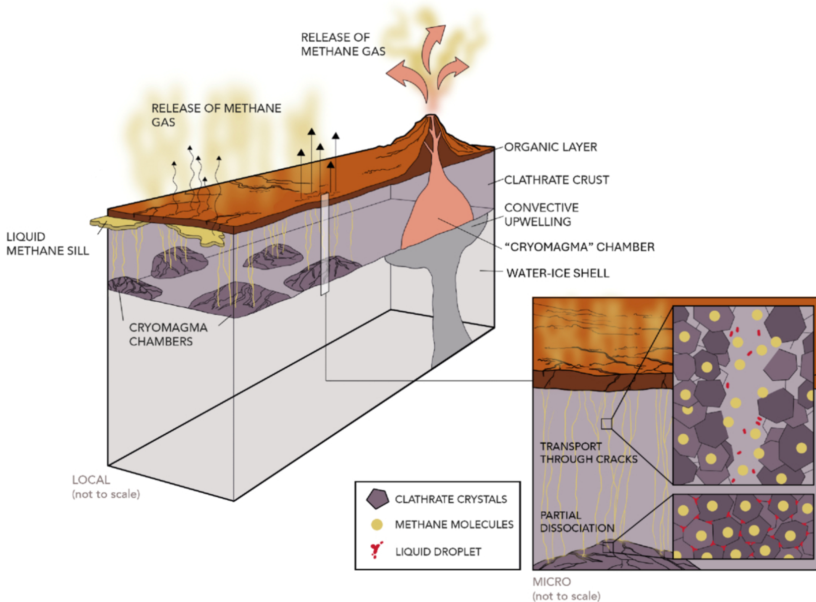
Figure 1. from Ashley Gerard Davies et al 2026 Planet. Sci. J. 7 doi:10.3847/PSJ/ae47df https://dx.doi.org/10.3847/PSJ/ae47df © 2026. The Author(s). Published by the American Astronomical Society.
