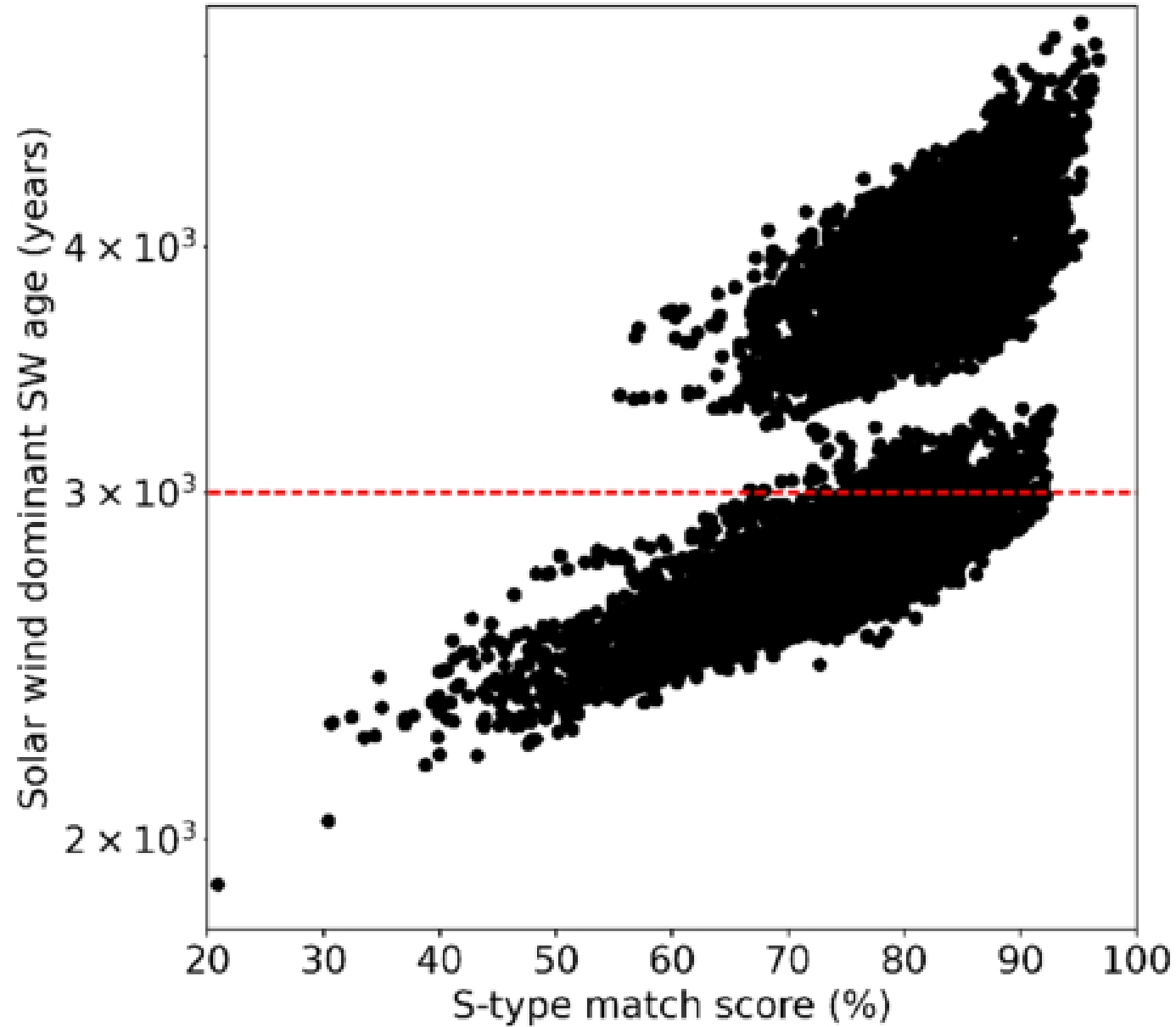
Figure 6. from Lakshika Palamakumbure et al 2026 Planet. Sci. J. 7 doi:10.3847/PSJ/ae4749 https://dx.doi.org/10.3847/PSJ/ae4749 © 2026. The Author(s). Published by the American Astronomical Society.
