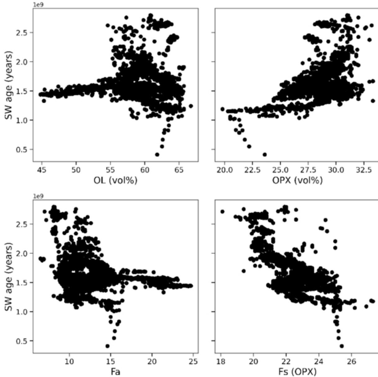
Figure 5. from Lakshika Palamakumbure et al 2026 Planet. Sci. J. 7 doi:10.3847/PSJ/ae4749 https://dx.doi.org/10.3847/PSJ/ae4749 © 2026. The Author(s). Published by the American Astronomical Society.
