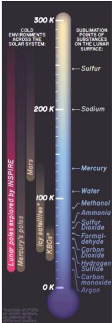
Figure 5. from Jennifer L. Heldmann et al 2026 Planet. Sci. J. 7 doi:10.3847/PSJ/ae4232 https://dx.doi.org/10.3847/PSJ/ae4232 © 2026. The Author(s). Published by the American Astronomical Society.
