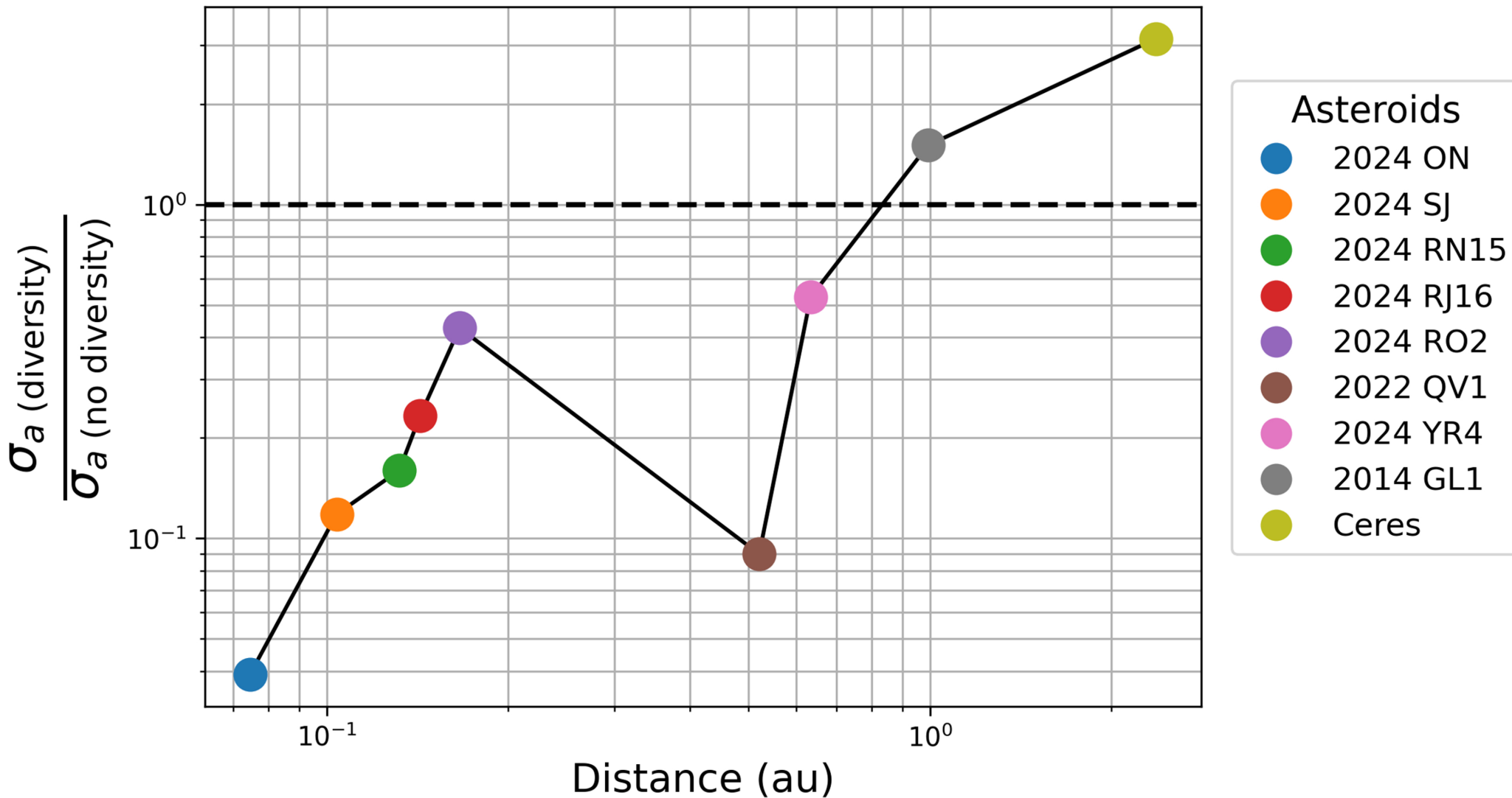
Figure 9. from Maryann Benny Fernandes et al 2026 Planet. Sci. J. 7 doi:10.3847/PSJ/ae2fe0 https://dx.doi.org/10.3847/PSJ/ae2fe0 © 2026. The Author(s). Published by the American Astronomical Society.
