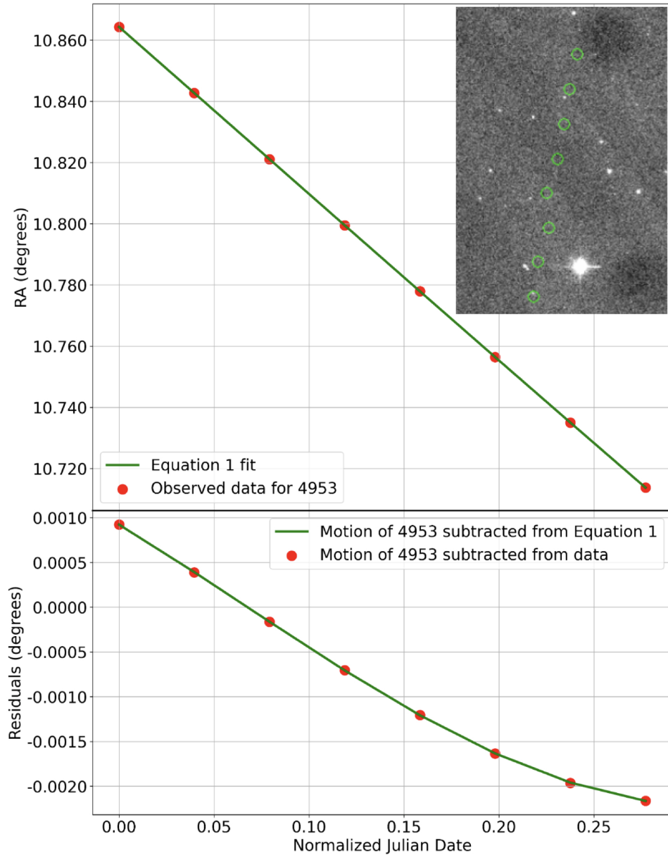
Figure 7. from Maryann Benny Fernandes et al 2026 Planet. Sci. J. 7 doi:10.3847/PSJ/ae2fe0 https://dx.doi.org/10.3847/PSJ/ae2fe0 © 2026. The Author(s). Published by the American Astronomical Society.
