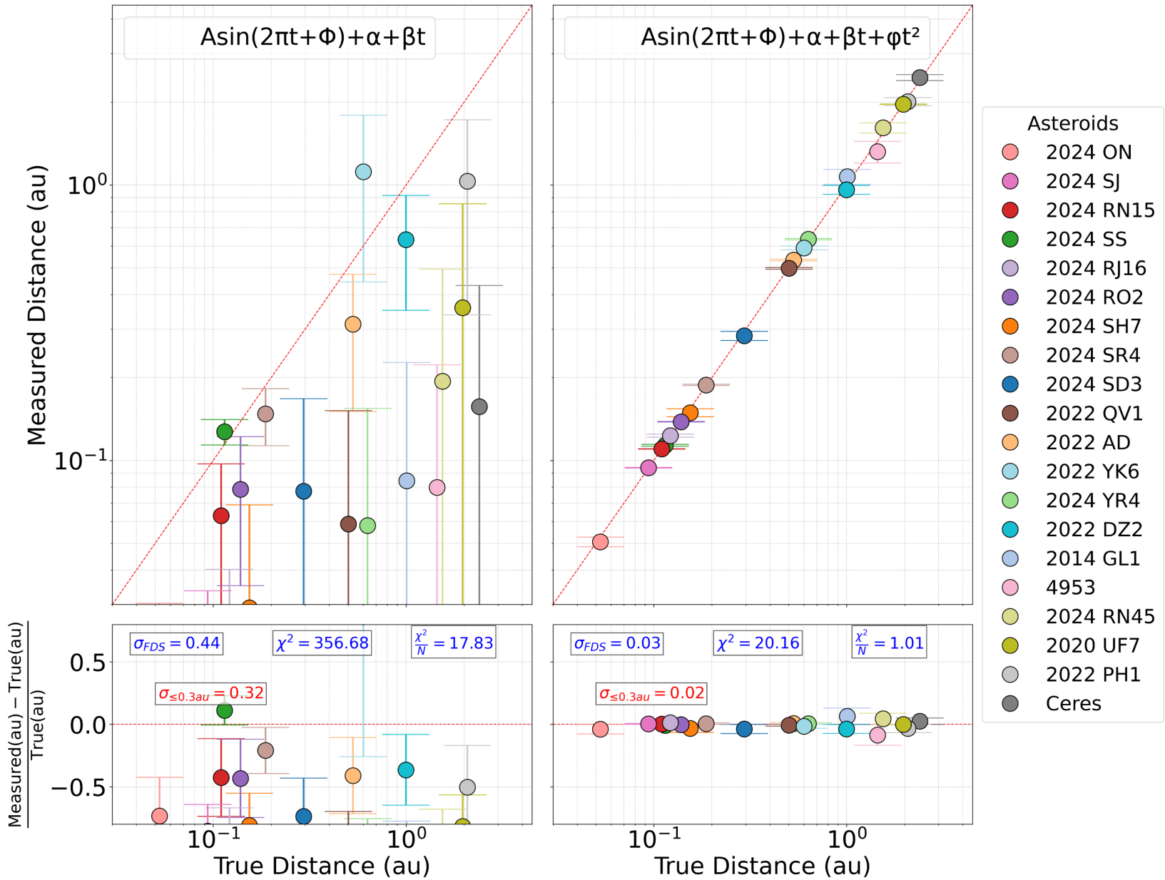
Figure 4. from Maryann Benny Fernandes et al 2026 Planet. Sci. J. 7 doi:10.3847/PSJ/ae2fe0 https://dx.doi.org/10.3847/PSJ/ae2fe0 © 2026. The Author(s). Published by the American Astronomical Society.
