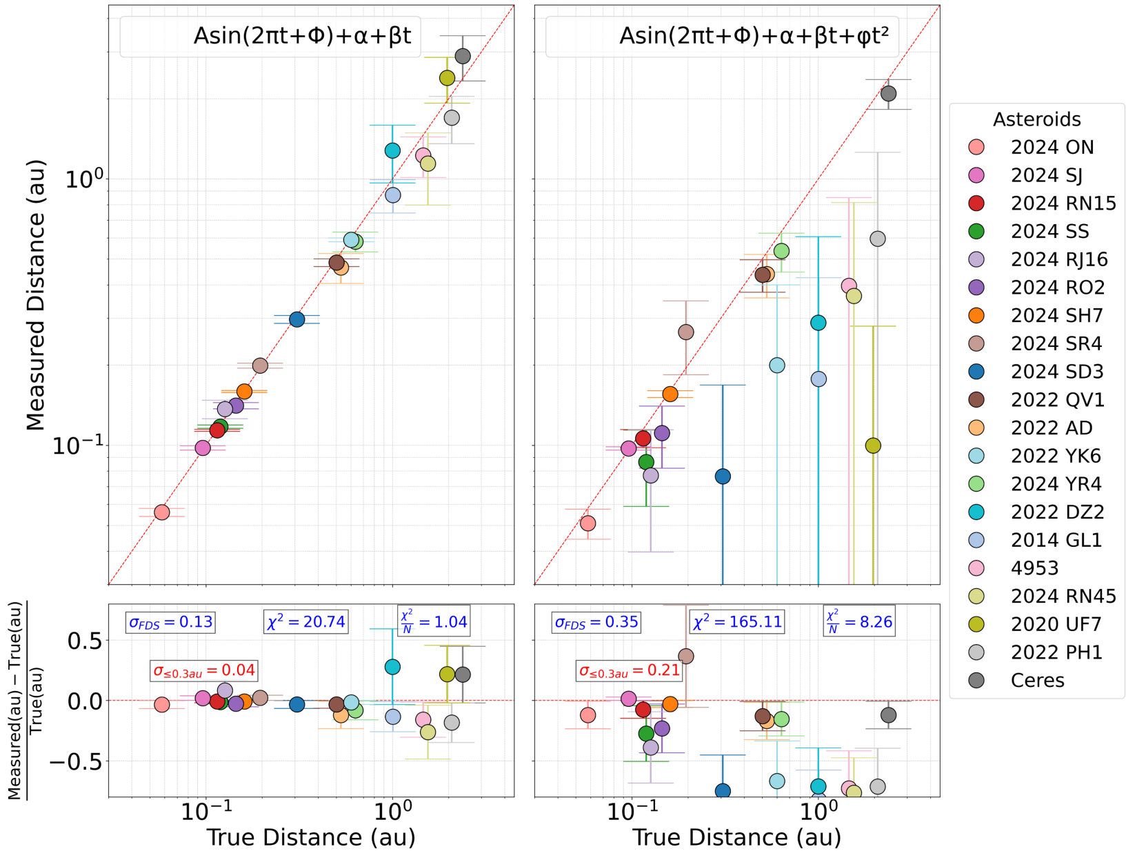
Figure 3. from Maryann Benny Fernandes et al 2026 Planet. Sci. J. 7 doi:10.3847/PSJ/ae2fe0 https://dx.doi.org/10.3847/PSJ/ae2fe0 © 2026. The Author(s). Published by the American Astronomical Society.
