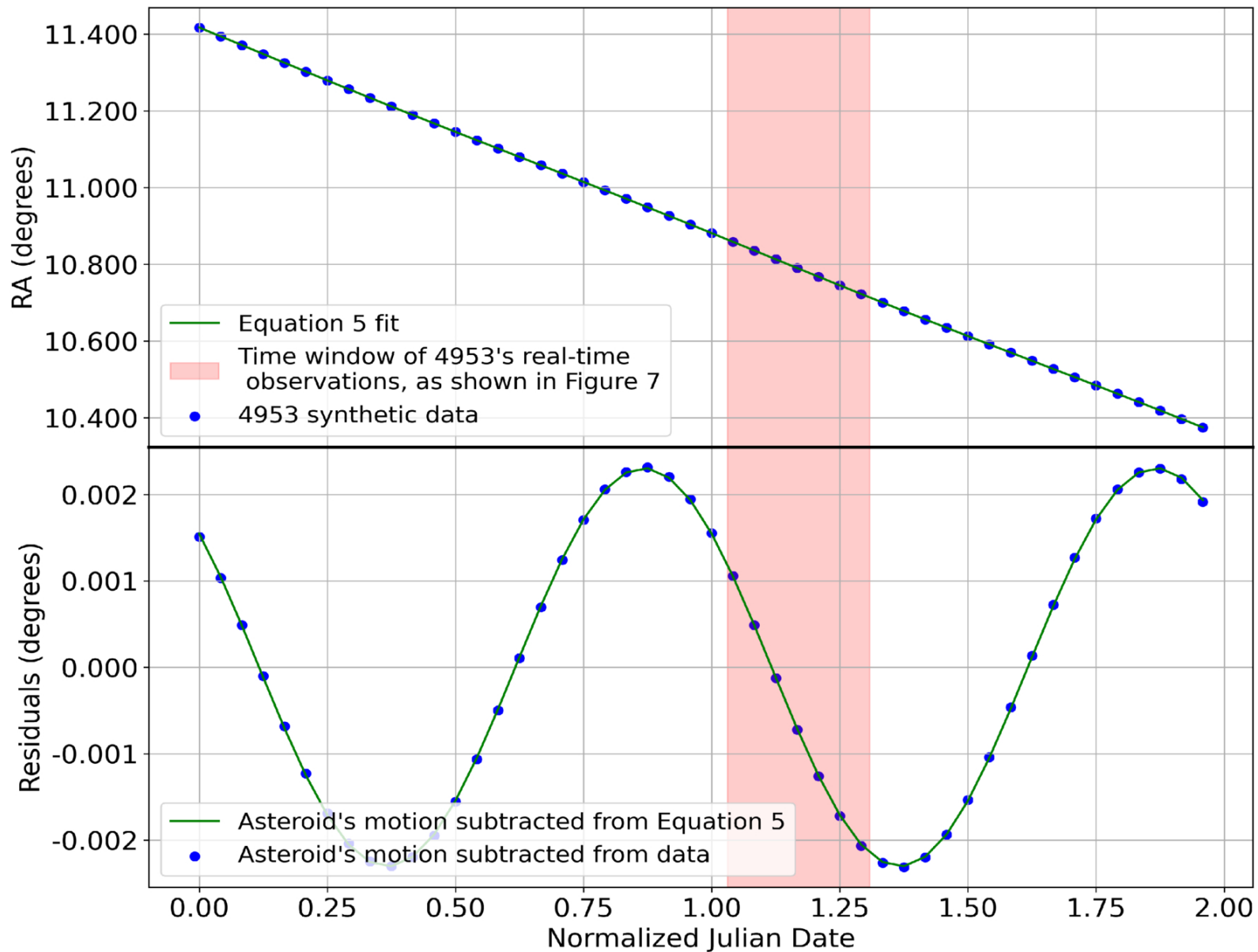
Figure 2. from Maryann Benny Fernandes et al 2026 Planet. Sci. J. 7 doi:10.3847/PSJ/ae2fe0 https://dx.doi.org/10.3847/PSJ/ae2fe0 © 2026. The Author(s). Published by the American Astronomical Society.
