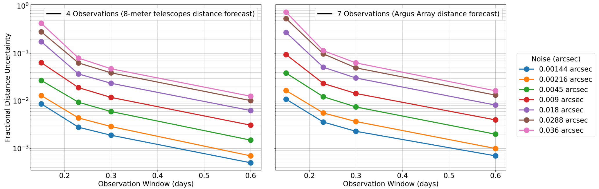
Figure 10. from Maryann Benny Fernandes et al 2026 Planet. Sci. J. 7 doi:10.3847/PSJ/ae2fe0 https://dx.doi.org/10.3847/PSJ/ae2fe0 © 2026. The Author(s). Published by the American Astronomical Society.
