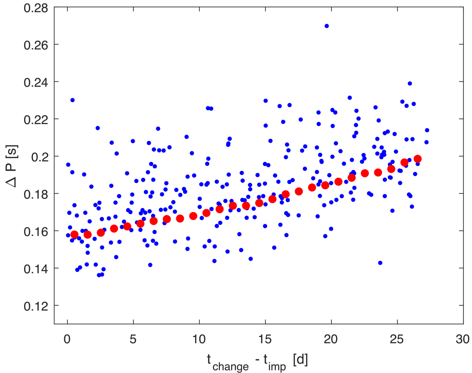
Figure 1. from Josef urech et al 2025 Planet. Sci. J. 6 doi:10.3847/PSJ/ae29ec https://dx.doi.org/10.3847/PSJ/ae29ec © 2025. The Author(s). Published by the American Astronomical Society.
