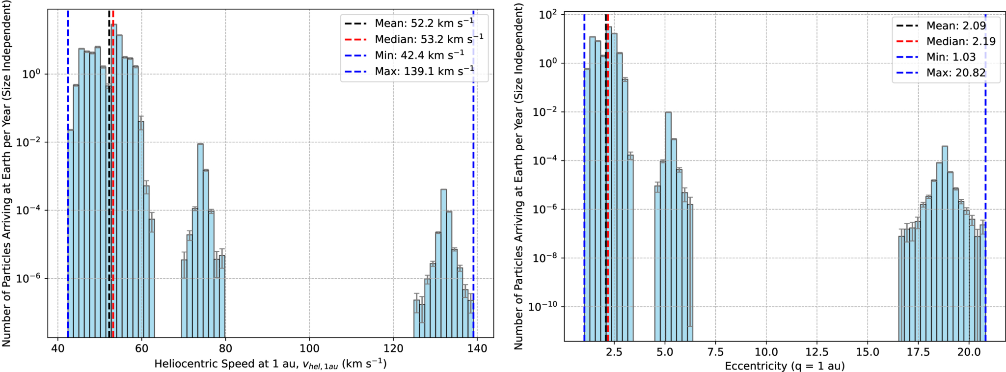
Figure 5. Heliocentric Velocity and Eccentricity Plots for All Systems from Cole R. Gregg and Paul A. Wiegert 2025 Planet. Sci. J. 6 doi:10.3847/PSJ/ae284f https://dx.doi.org/10.3847/PSJ/ae284f © 2025. The Author(s). Published by the American Astronomical Society.
