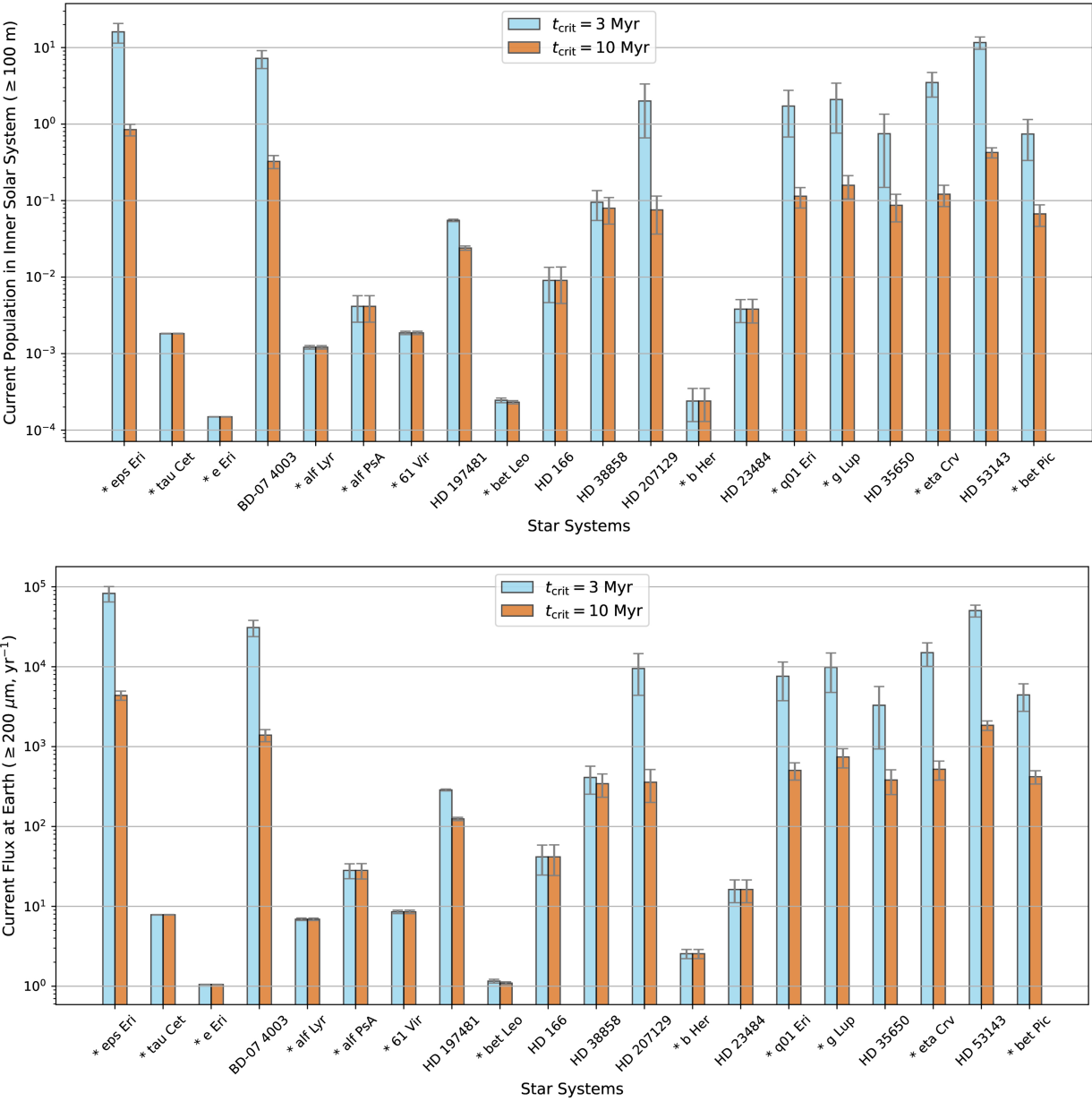
Figure 3. from Cole R. Gregg and Paul A. Wiegert 2025 Planet. Sci. J. 6 doi:10.3847/PSJ/ae284f https://dx.doi.org/10.3847/PSJ/ae284f © 2025. The Author(s). Published by the American Astronomical Society.
