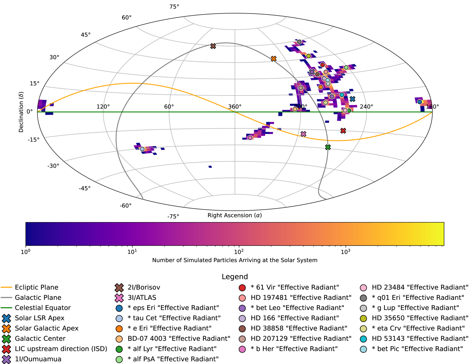
Figure 2. Radiant Heatmaps for All Systems from Cole R. Gregg and Paul A. Wiegert 2025 Planet. Sci. J. 6 doi:10.3847/PSJ/ae284f https://dx.doi.org/10.3847/PSJ/ae284f © 2025. The Author(s). Published by the American Astronomical Society.
