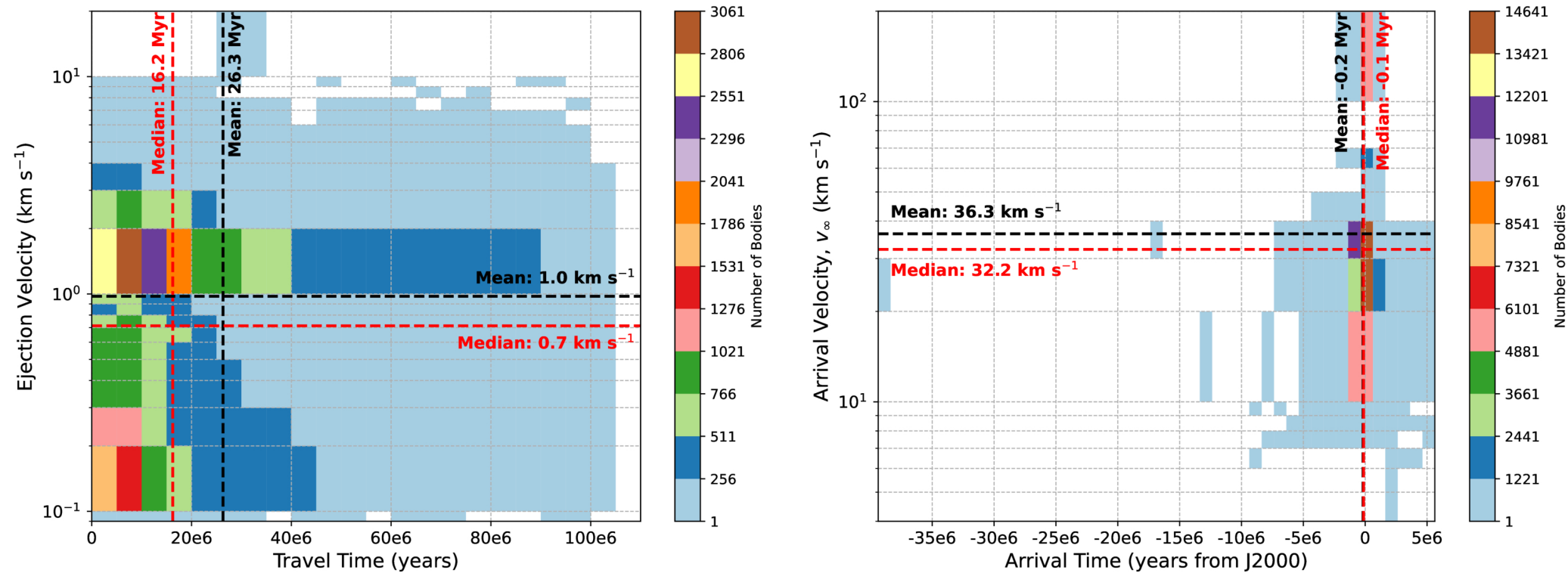
Figure 1. Arrival and Travel Heatplots for All Systems from Cole R. Gregg and Paul A. Wiegert 2025 Planet. Sci. J. 6 doi:10.3847/PSJ/ae284f https://dx.doi.org/10.3847/PSJ/ae284f © 2025. The Author(s). Published by the American Astronomical Society.
