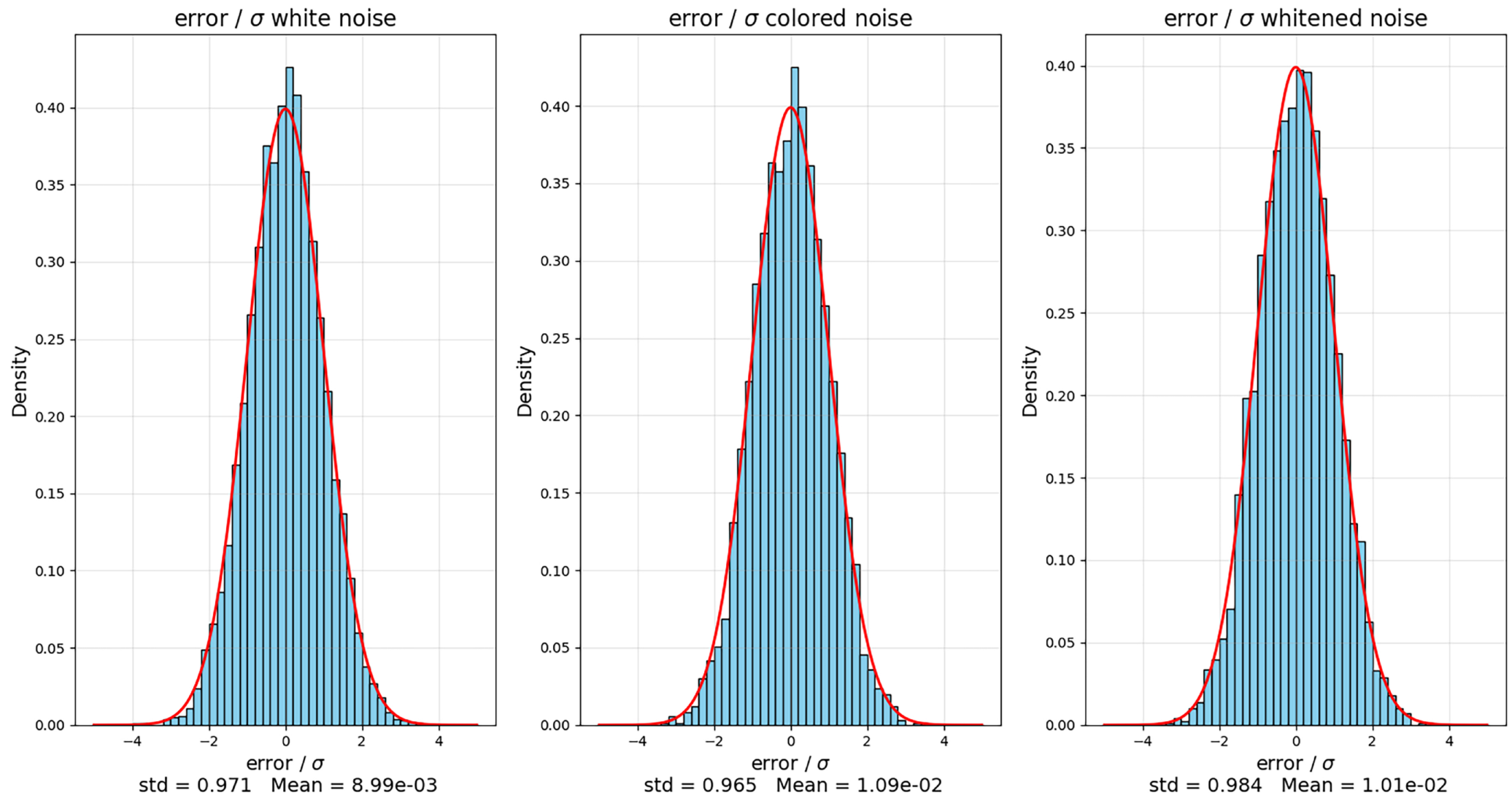
Figure 8. from Flavia Giuliani et al 2026 Planet. Sci. J. 7 doi:10.3847/PSJ/ae1fda https://dx.doi.org/10.3847/PSJ/ae1fda © 2026. The Author(s). Published by the American Astronomical Society.
