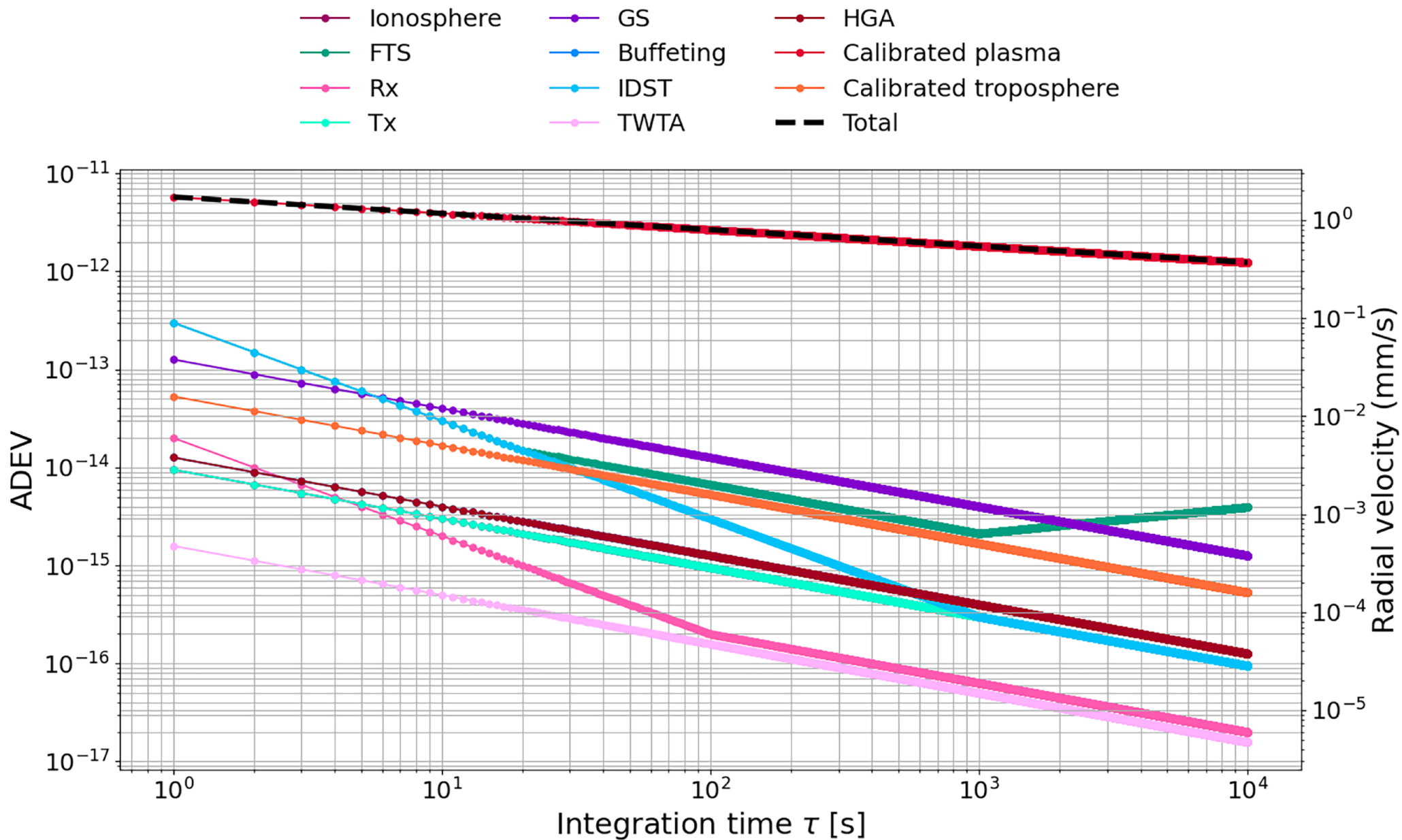
Figure 2. from Flavia Giuliani et al 2026 Planet. Sci. J. 7 doi:10.3847/PSJ/ae1fda https://dx.doi.org/10.3847/PSJ/ae1fda © 2026. The Author(s). Published by the American Astronomical Society.
