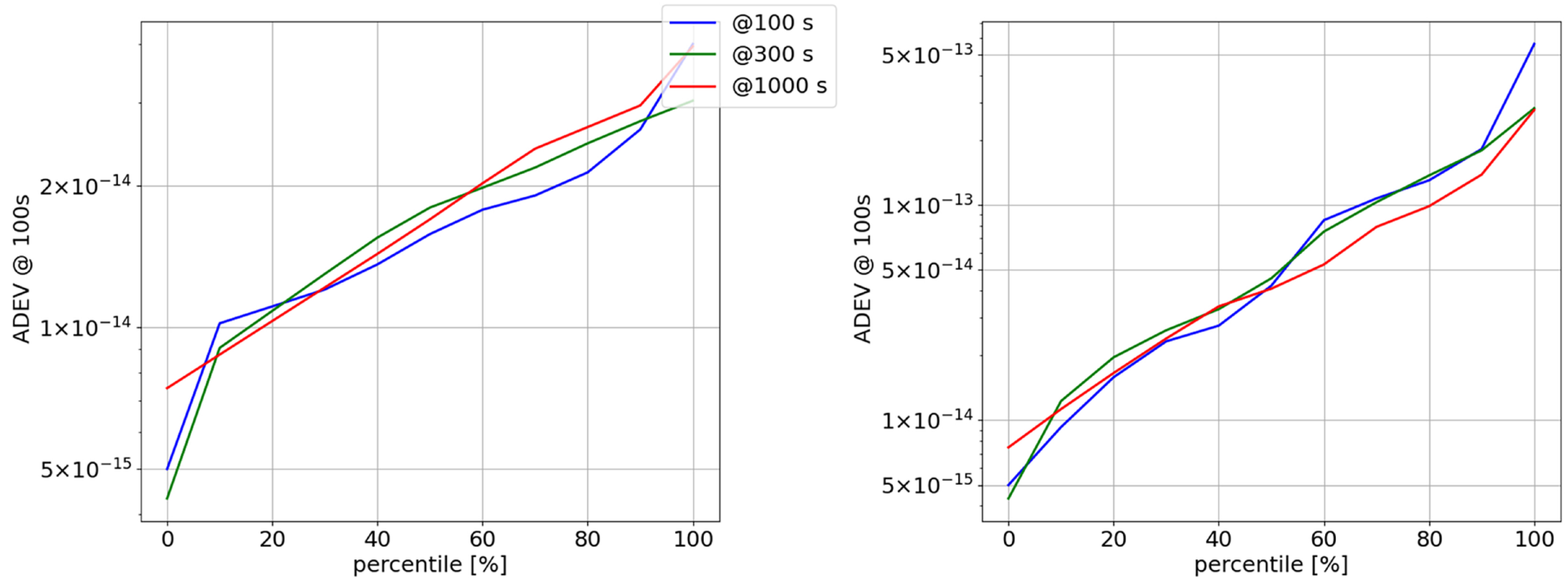
Figure 14. from Flavia Giuliani et al 2026 Planet. Sci. J. 7 doi:10.3847/PSJ/ae1fda https://dx.doi.org/10.3847/PSJ/ae1fda © 2026. The Author(s). Published by the American Astronomical Society.
