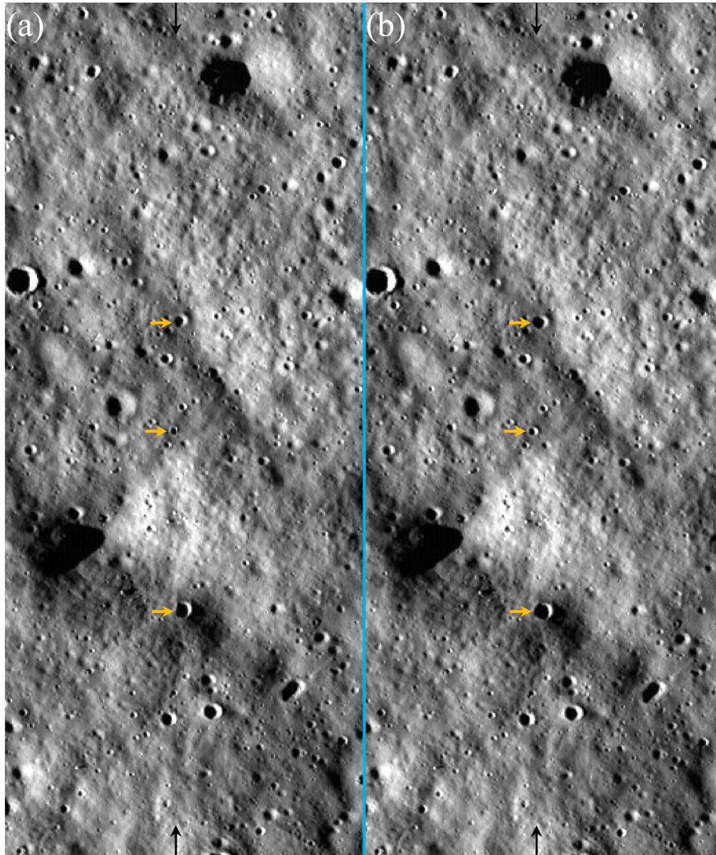
Figure 6. from Ryodo Hemmi et al 2025 Planet. Sci. J. 6 doi:10.3847/PSJ/ae10a4 https://dx.doi.org/10.3847/PSJ/ae10a4 © 2025. The Author(s). Published by the American Astronomical Society.
