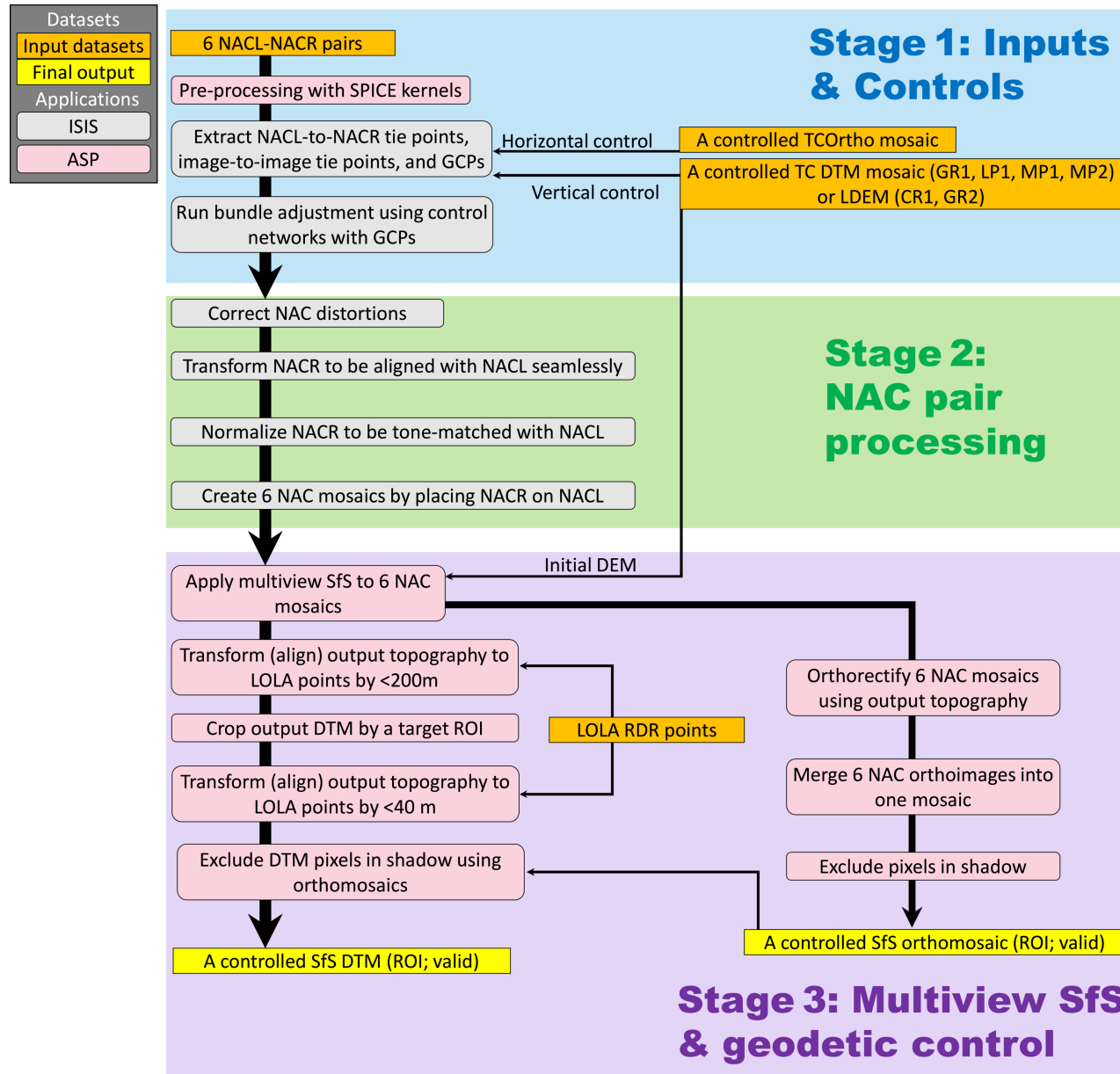
Figure 5. from Ryodo Hemmi et al 2025 Planet. Sci. J. 6 doi:10.3847/PSJ/ae10a4 https://dx.doi.org/10.3847/PSJ/ae10a4 © 2025. The Author(s). Published by the American Astronomical Society.
