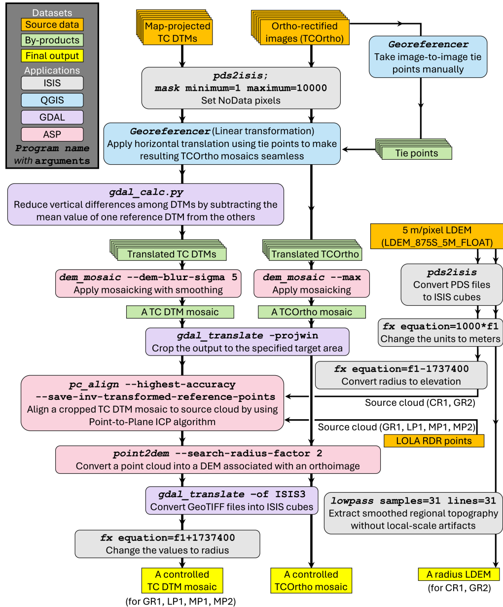
Figure 4. from Ryodo Hemmi et al 2025 Planet. Sci. J. 6 doi:10.3847/PSJ/ae10a4 https://dx.doi.org/10.3847/PSJ/ae10a4 © 2025. The Author(s). Published by the American Astronomical Society.
