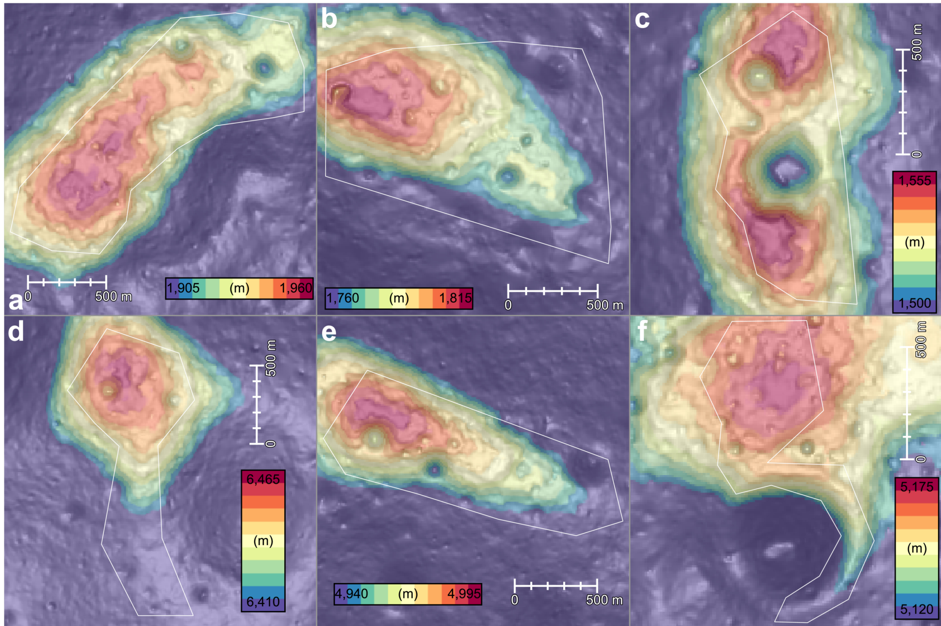
Figure 3. from Ryodo Hemmi et al 2025 Planet. Sci. J. 6 doi:10.3847/PSJ/ae10a4 https://dx.doi.org/10.3847/PSJ/ae10a4 © 2025. The Author(s). Published by the American Astronomical Society.
