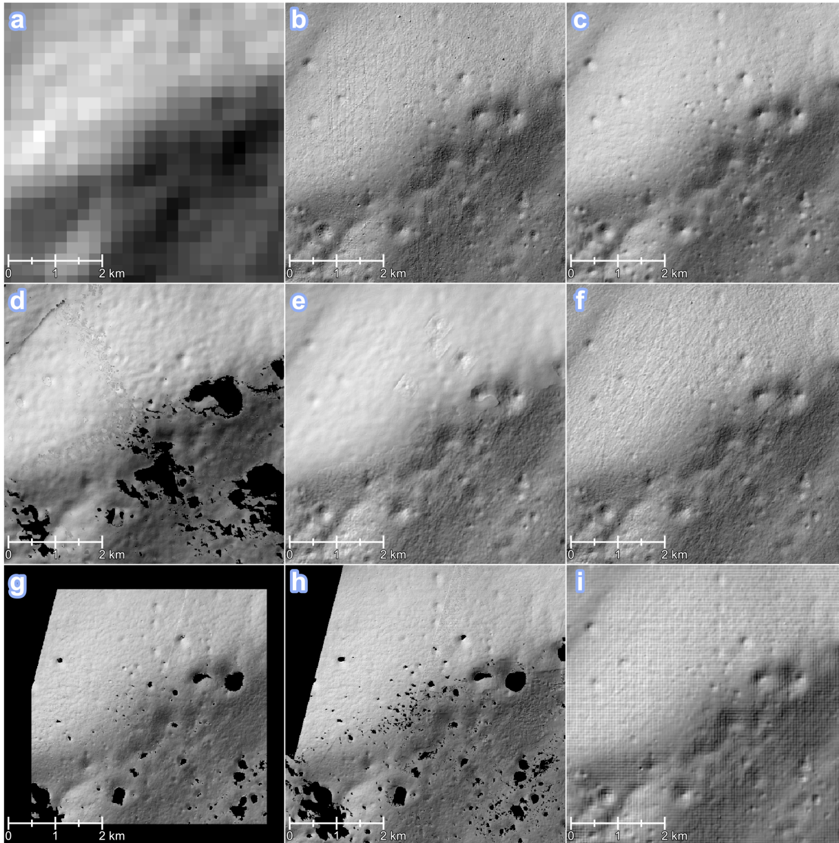
Figure 2. from Ryodo Hemmi et al 2025 Planet. Sci. J. 6 doi:10.3847/PSJ/ae10a4 https://dx.doi.org/10.3847/PSJ/ae10a4 © 2025. The Author(s). Published by the American Astronomical Society.
