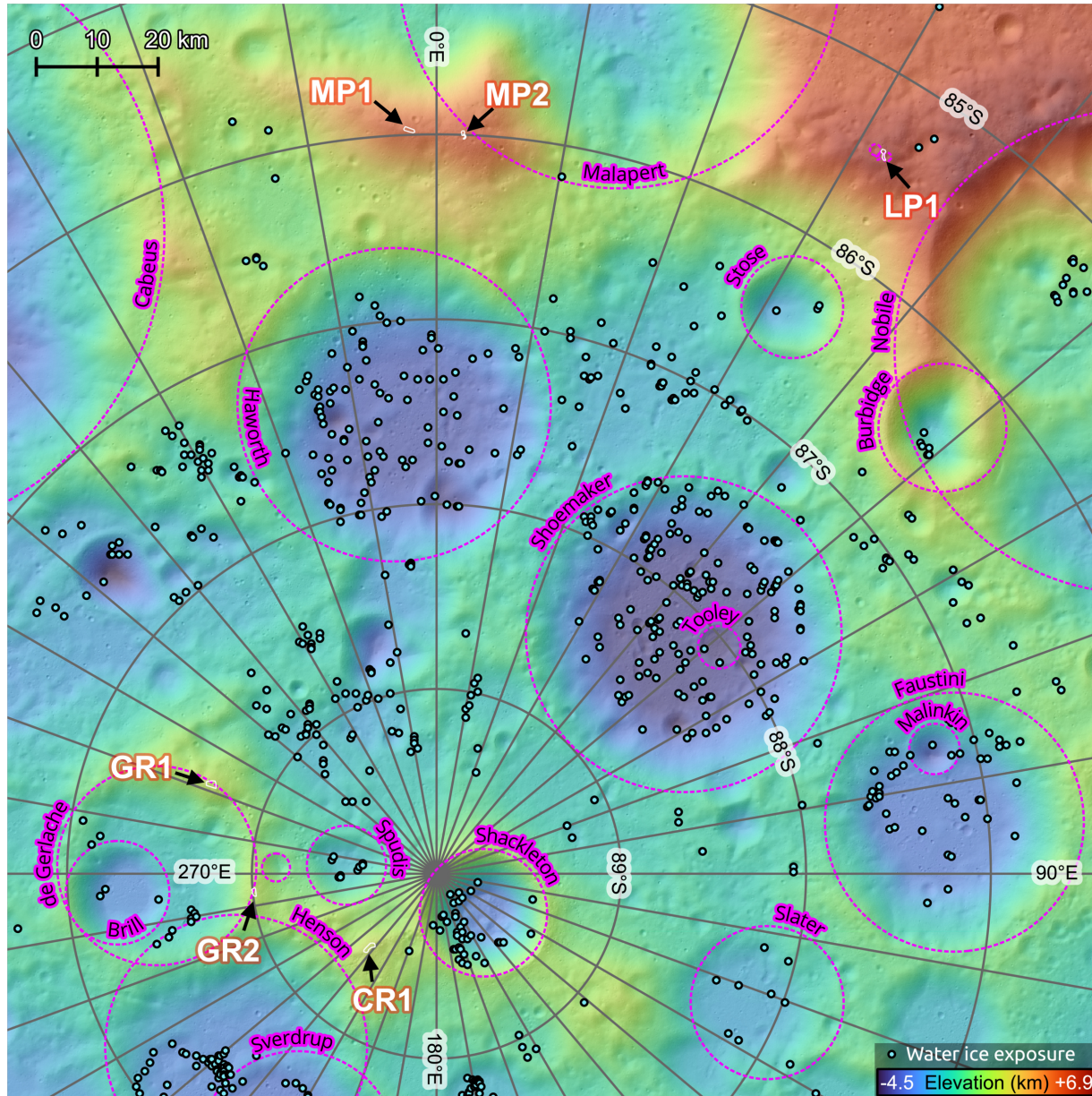
Figure 1. from Ryodo Hemmi et al 2025 Planet. Sci. J. 6 doi:10.3847/PSJ/ae10a4 https://dx.doi.org/10.3847/PSJ/ae10a4 © 2025. The Author(s). Published by the American Astronomical Society.
