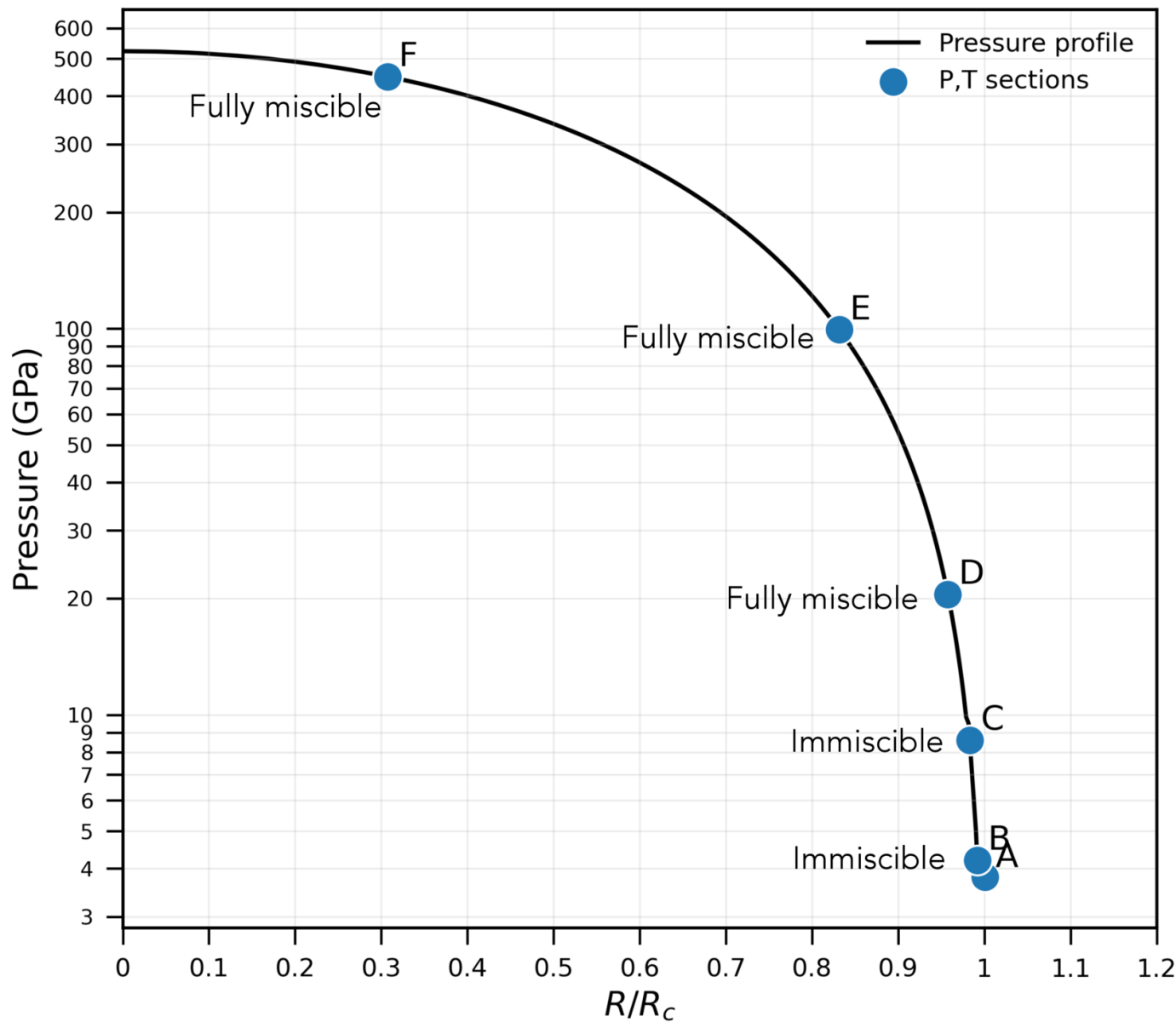
Figure 9. from Edward D. Young et al 2025 Planet. Sci. J. 6 doi:10.3847/PSJ/ae1012 https://dx.doi.org/10.3847/PSJ/ae1012 © 2025. The Author(s). Published by the American Astronomical Society.
