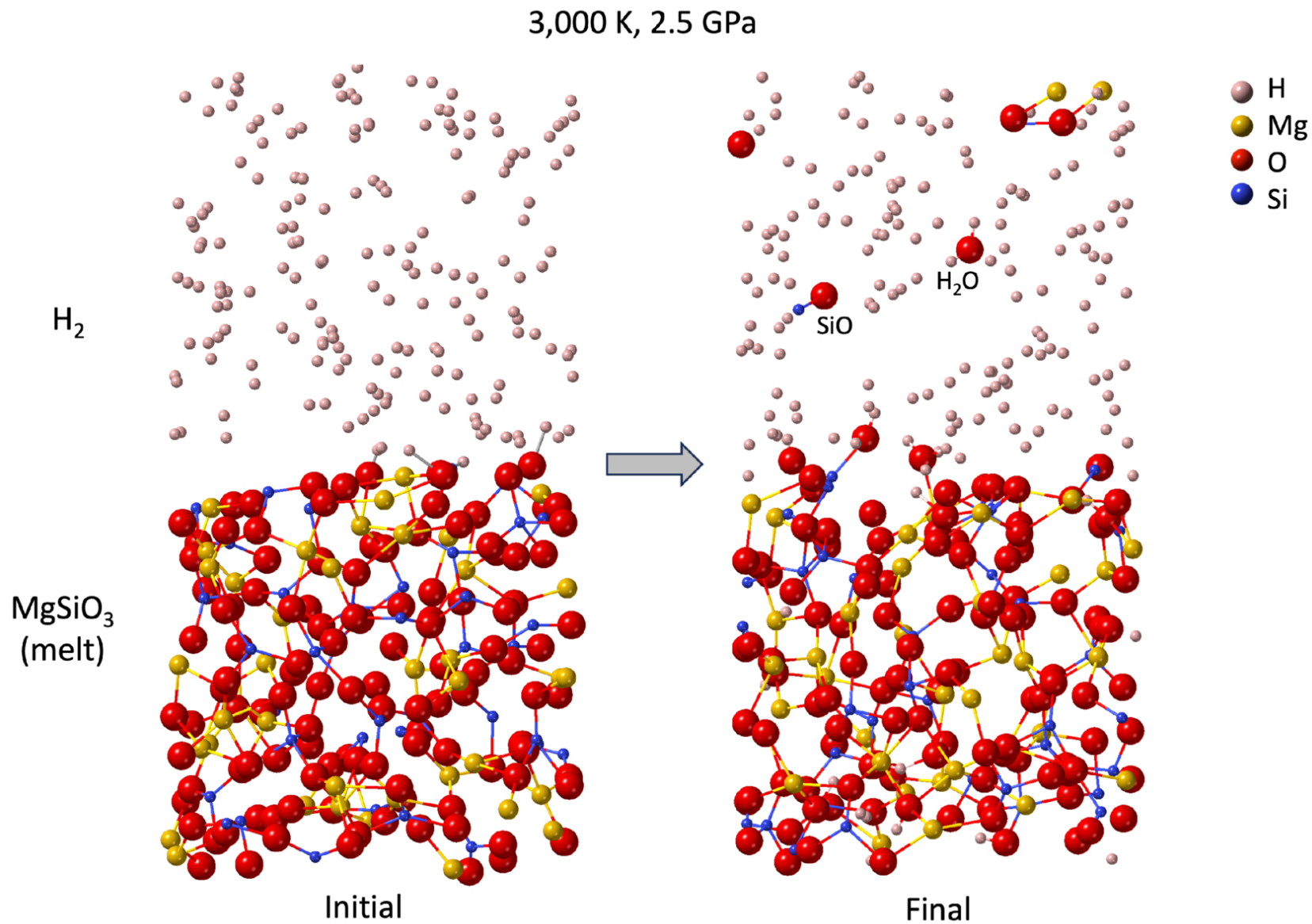
Figure 4. from Edward D. Young et al 2025 Planet. Sci. J. 6 doi:10.3847/PSJ/ae1012 https://dx.doi.org/10.3847/PSJ/ae1012 © 2025. The Author(s). Published by the American Astronomical Society.
