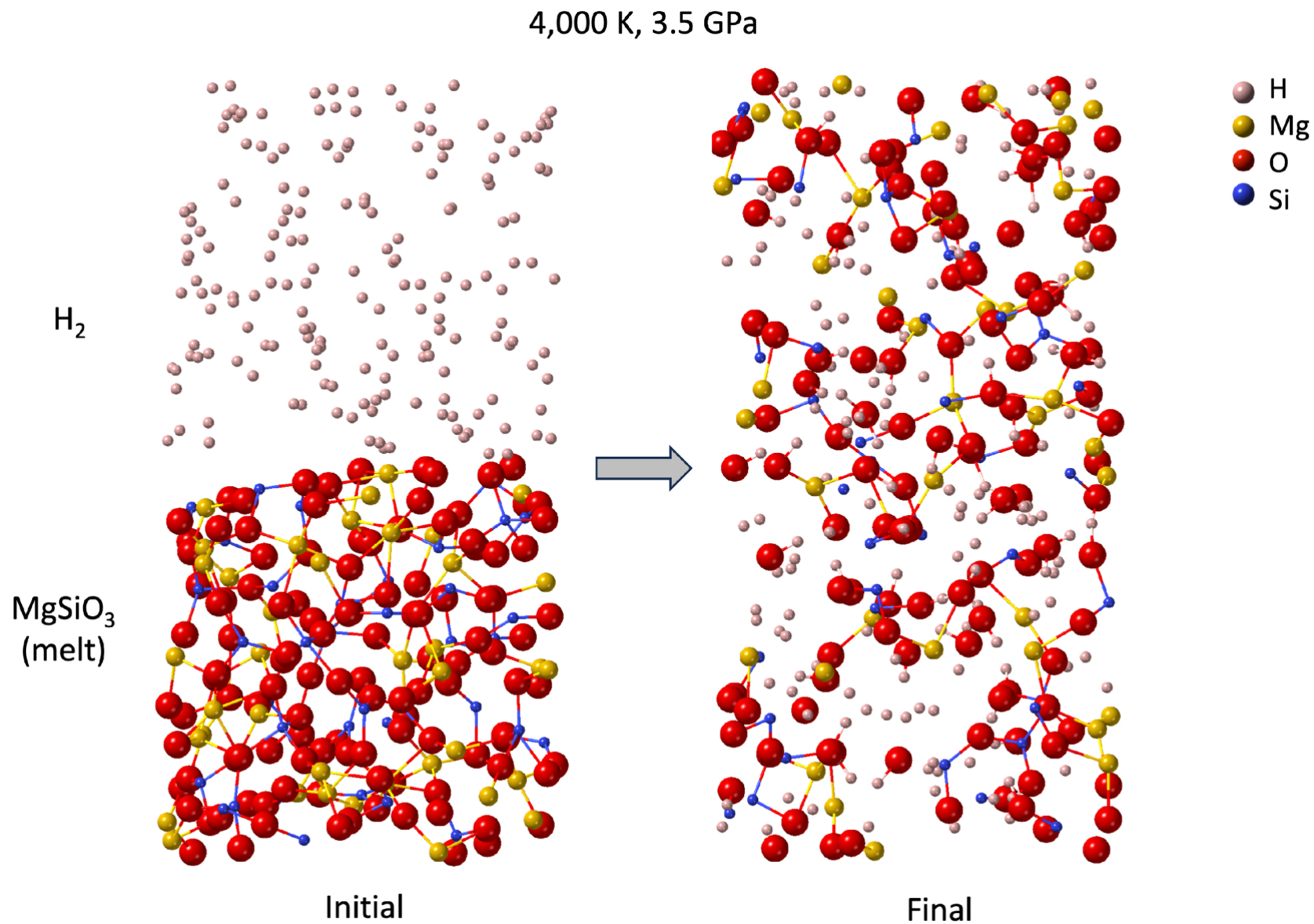
Figure 3. from Edward D. Young et al 2025 Planet. Sci. J. 6 doi:10.3847/PSJ/ae1012 https://dx.doi.org/10.3847/PSJ/ae1012 © 2025. The Author(s). Published by the American Astronomical Society.
