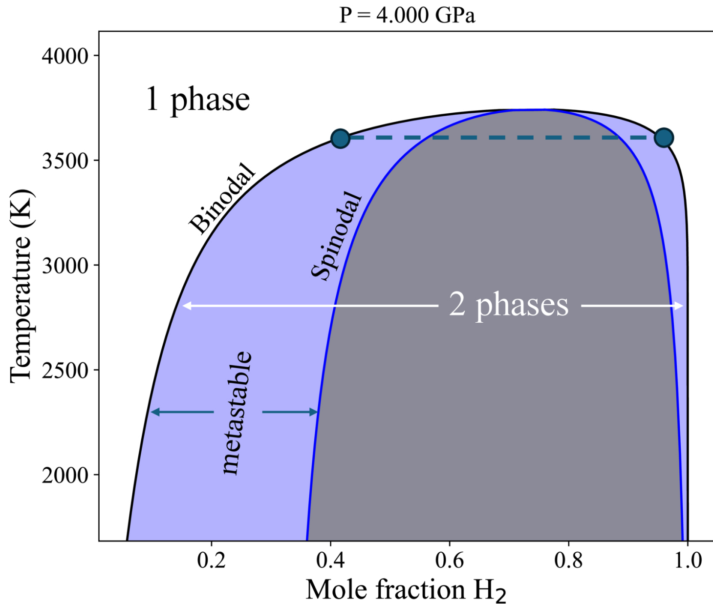
Figure 2. from Edward D. Young et al 2025 Planet. Sci. J. 6 doi:10.3847/PSJ/ae1012 https://dx.doi.org/10.3847/PSJ/ae1012 © 2025. The Author(s). Published by the American Astronomical Society.
