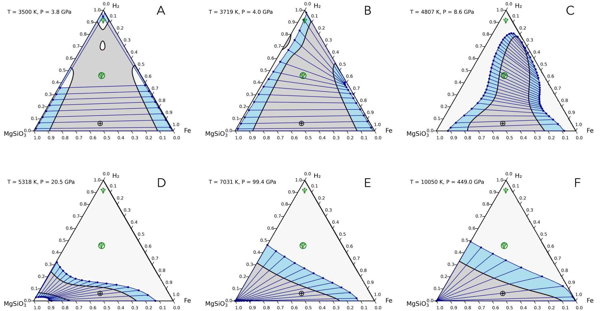
Figure 10. from Edward D. Young et al 2025 Planet. Sci. J. 6 doi:10.3847/PSJ/ae1012 https://dx.doi.org/10.3847/PSJ/ae1012 © 2025. The Author(s). Published by the American Astronomical Society.
