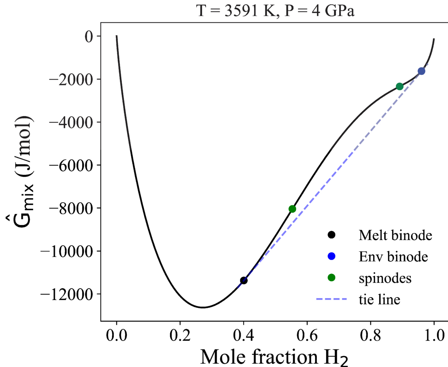
Figure 1. from Edward D. Young et al 2025 Planet. Sci. J. 6 doi:10.3847/PSJ/ae1012 https://dx.doi.org/10.3847/PSJ/ae1012 © 2025. The Author(s). Published by the American Astronomical Society.
