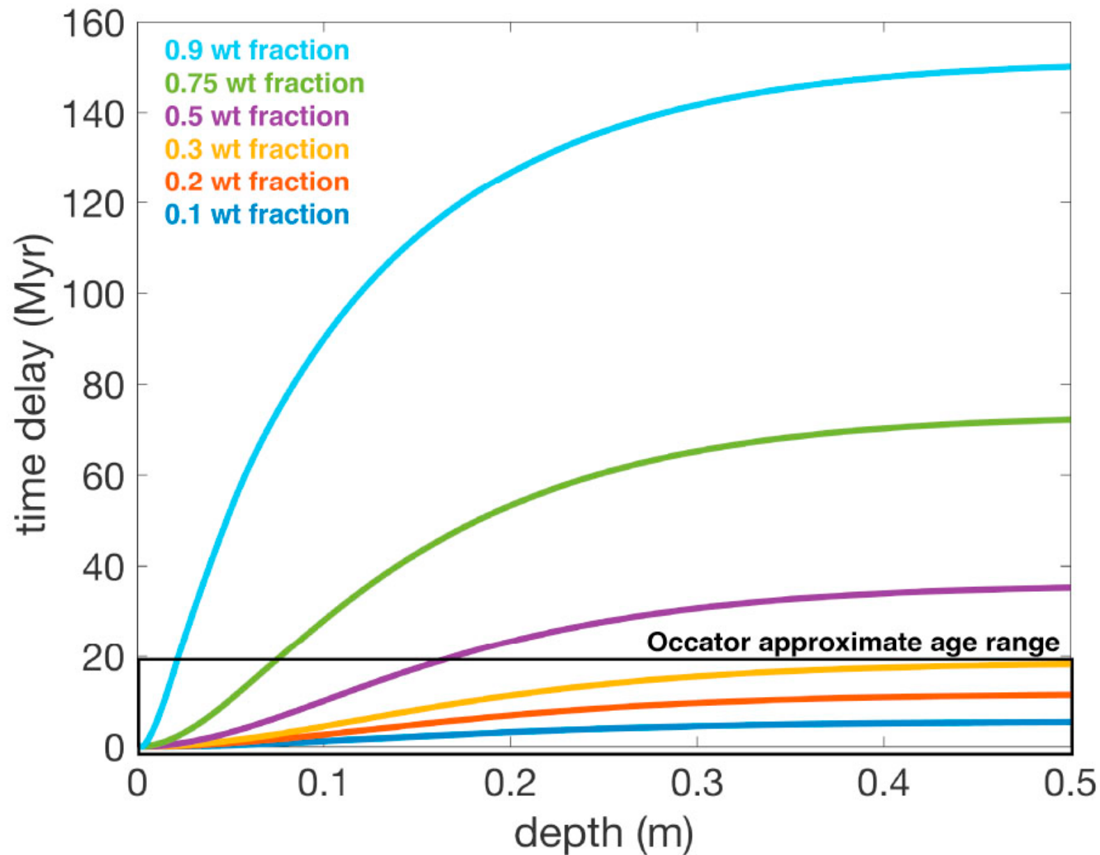
Figure 2. from Margaret E. Landis et al 2025 Planet. Sci. J. 6 doi:10.3847/PSJ/ae0333 https://dx.doi.org/10.3847/PSJ/ae0333 © 2025. The Author(s). Published by the American Astronomical Society.
