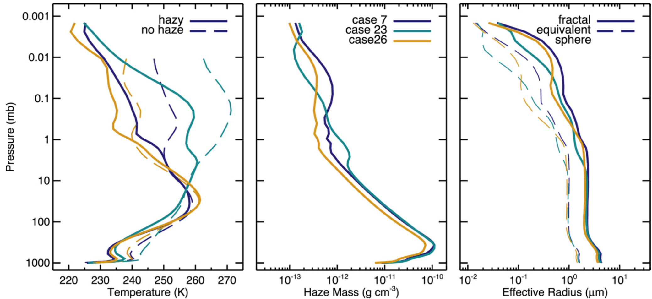
Figure 7. from Eric T. Wolf et al 2025 Planet. Sci. J. 6 doi:10.3847/PSJ/ae031e https://dx.doi.org/10.3847/PSJ/ae031e © 2025. The Author(s). Published by the American Astronomical Society.
