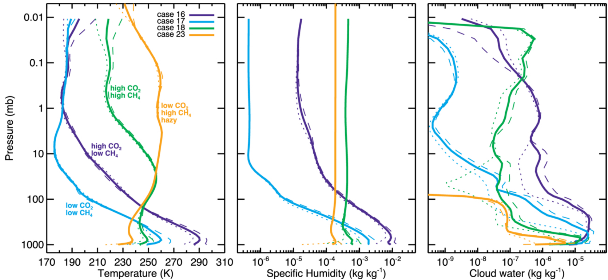
Figure 6. from Eric T. Wolf et al 2025 Planet. Sci. J. 6 doi:10.3847/PSJ/ae031e https://dx.doi.org/10.3847/PSJ/ae031e © 2025. The Author(s). Published by the American Astronomical Society.
