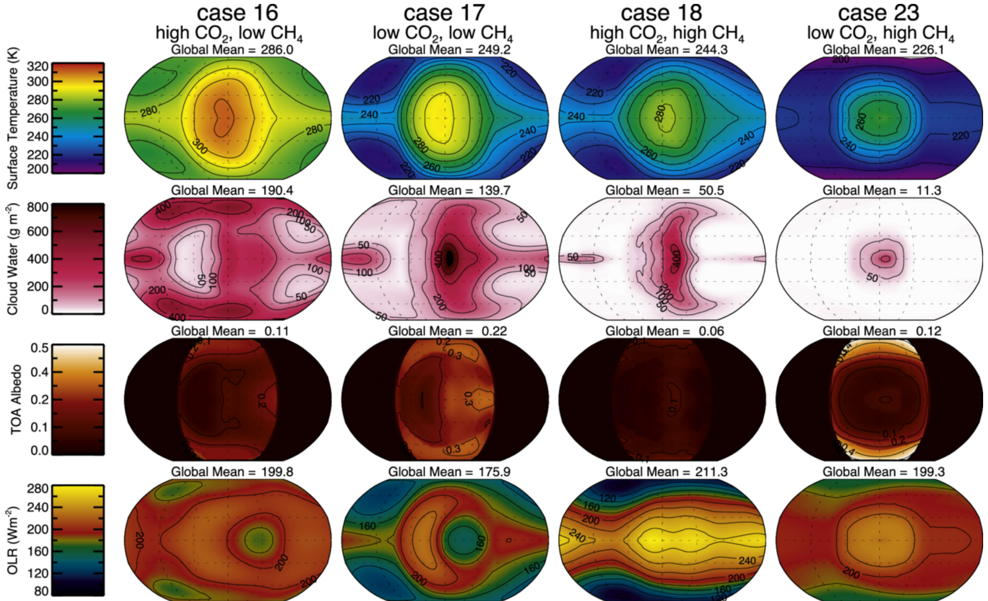
Figure 5. from Eric T. Wolf et al 2025 Planet. Sci. J. 6 doi:10.3847/PSJ/ae031e https://dx.doi.org/10.3847/PSJ/ae031e © 2025. The Author(s). Published by the American Astronomical Society.
