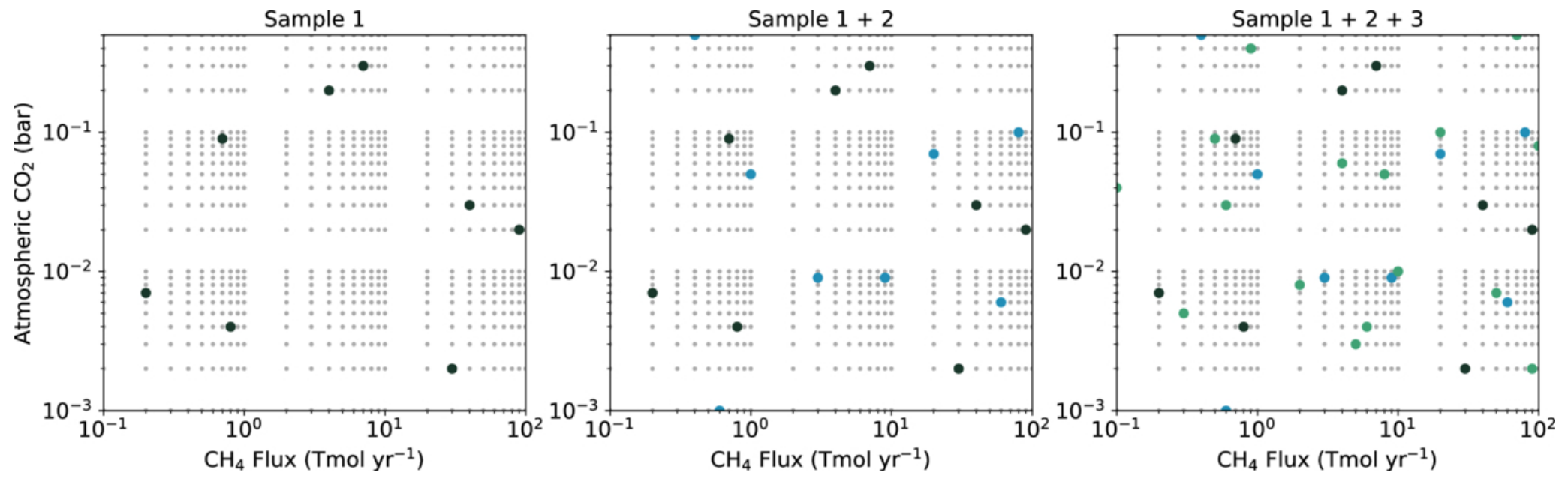
Figure 2. from Eric T. Wolf et al 2025 Planet. Sci. J. 6 doi:10.3847/PSJ/ae031e https://dx.doi.org/10.3847/PSJ/ae031e © 2025. The Author(s). Published by the American Astronomical Society.
