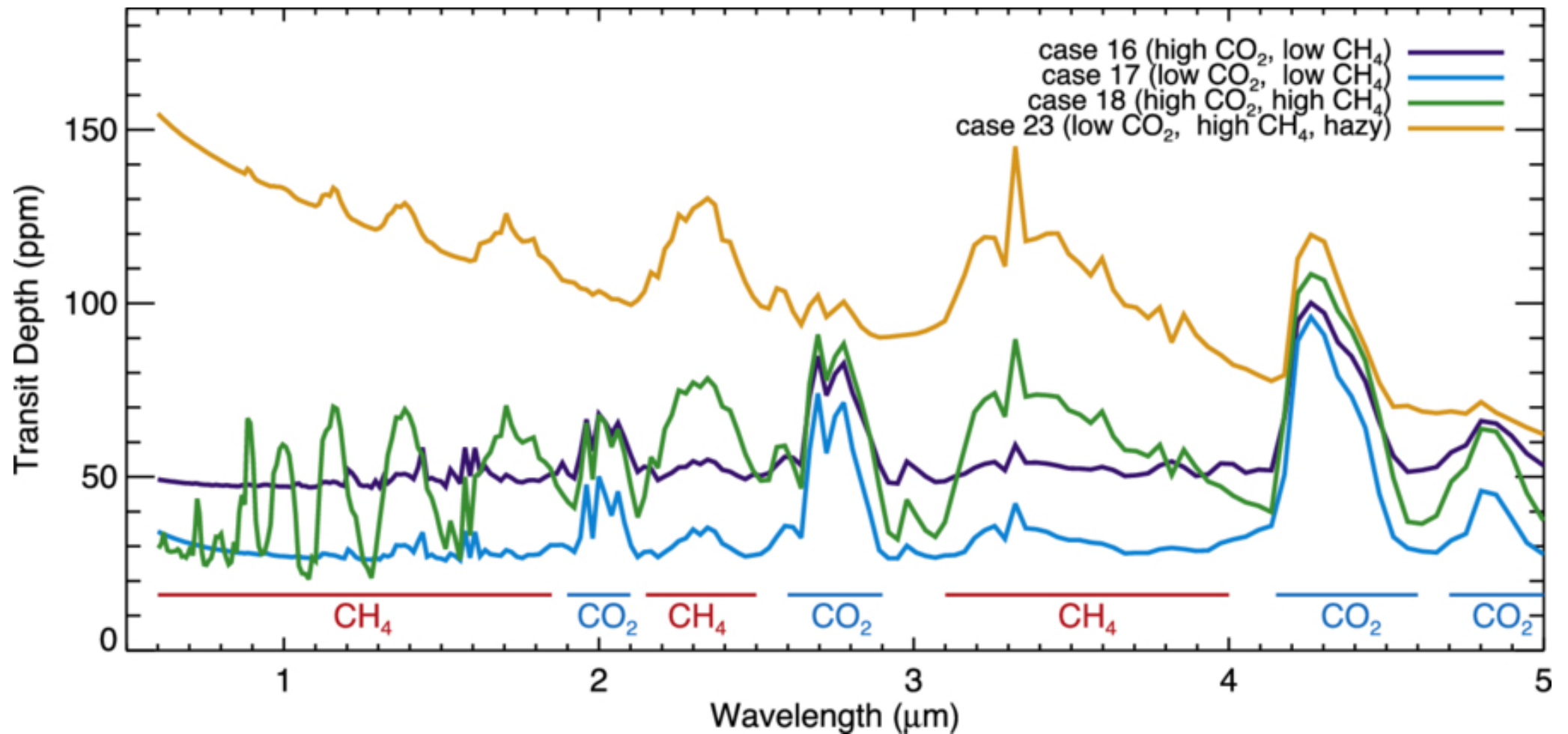
Figure 10. from Eric T. Wolf et al 2025 Planet. Sci. J. 6 doi:10.3847/PSJ/ae031e https://dx.doi.org/10.3847/PSJ/ae031e © 2025. The Author(s). Published by the American Astronomical Society.
