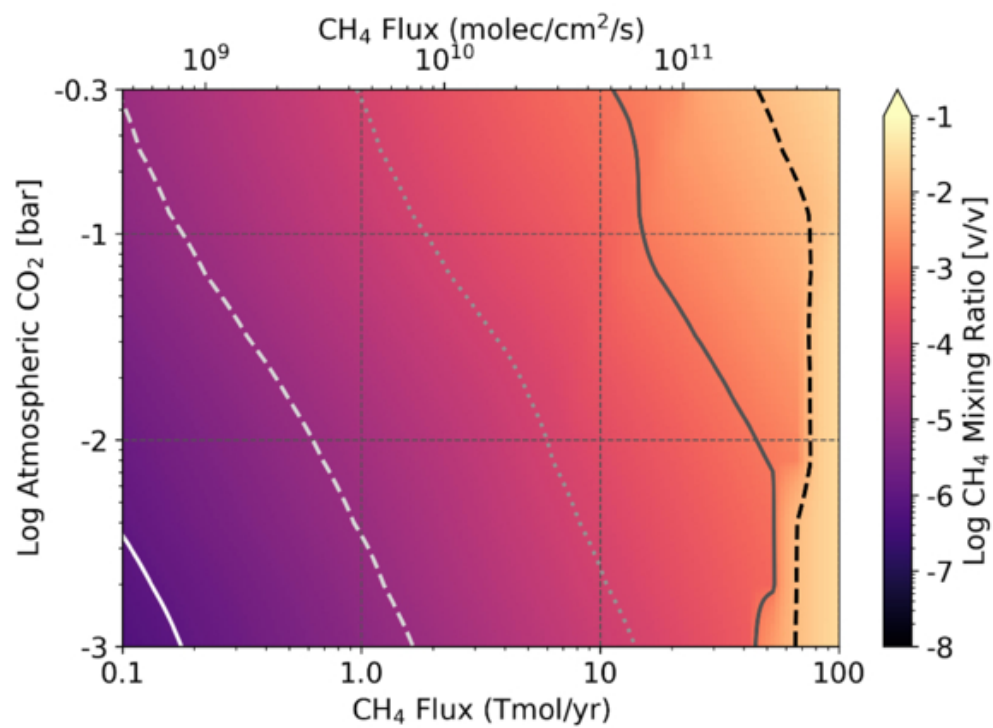
Figure 1. from Eric T. Wolf et al 2025 Planet. Sci. J. 6 doi:10.3847/PSJ/ae031e https://dx.doi.org/10.3847/PSJ/ae031e © 2025. The Author(s). Published by the American Astronomical Society.
