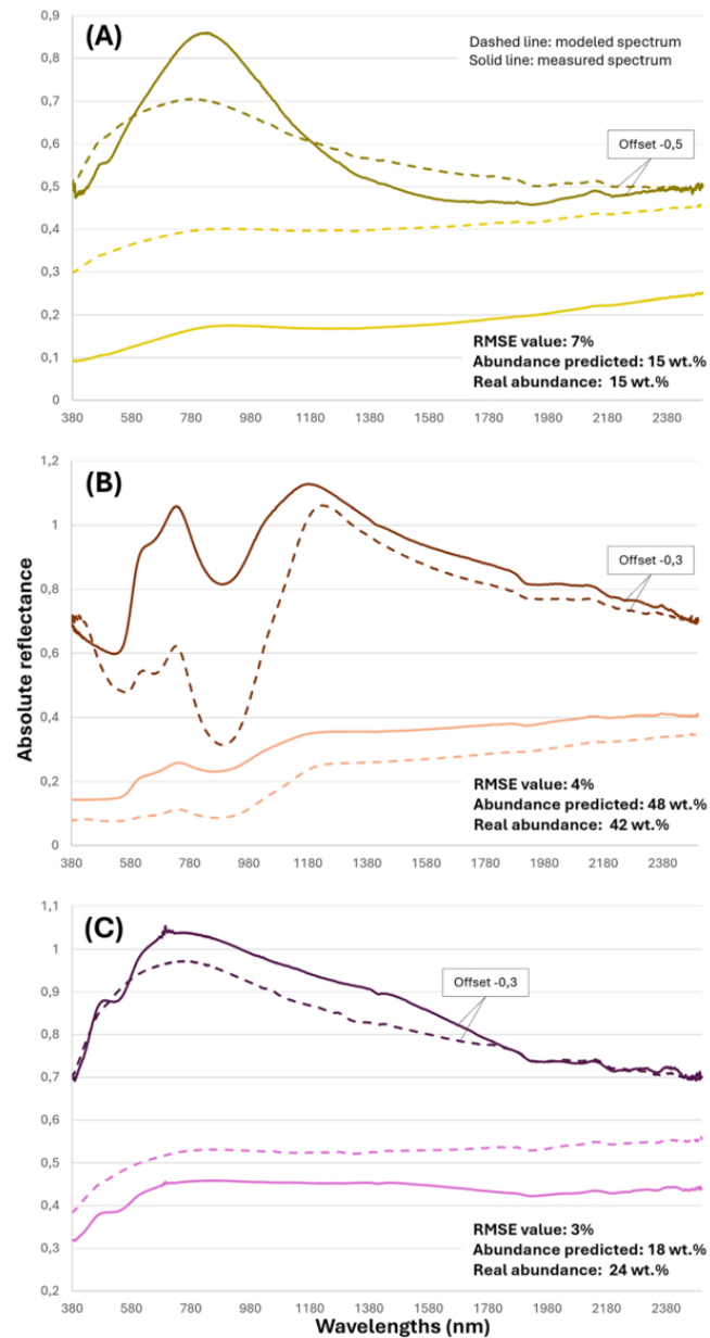
Figure 6. from Alex Camon and Myriam Lemelin 2025 Planet. Sci. J. 6 doi:10.3847/PSJ/adee0c https://dx.doi.org/10.3847/PSJ/adee0c © 2025. The Author(s). Published by the American Astronomical Society.
