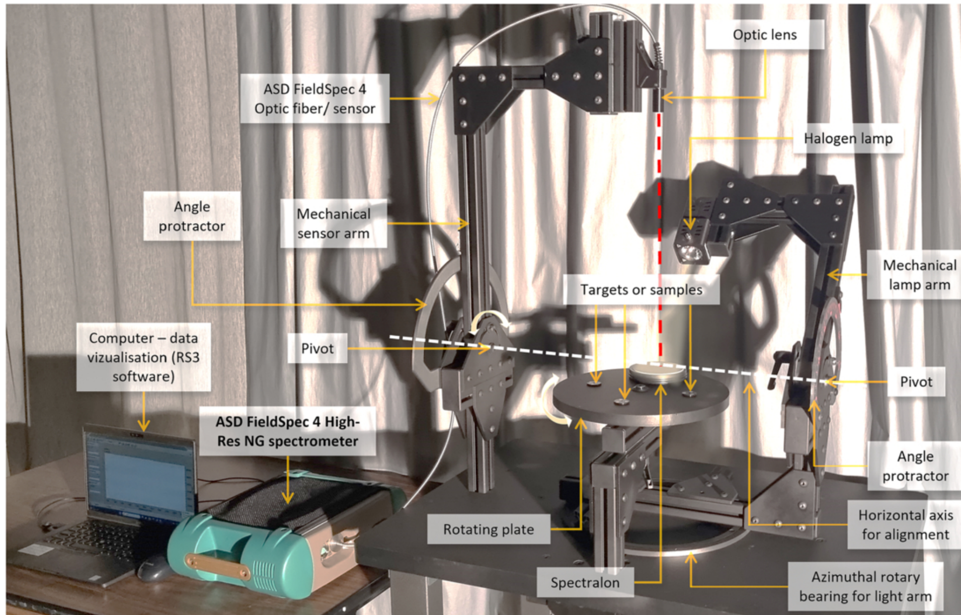
Figure 1. from Alex Camon and Myriam Lemelin 2025 Planet. Sci. J. 6 doi:10.3847/PSJ/adee0c https://dx.doi.org/10.3847/PSJ/adee0c © 2025. The Author(s). Published by the American Astronomical Society.
